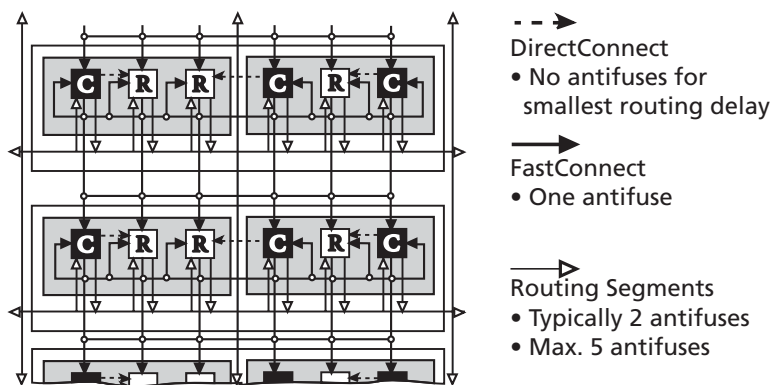
Figure 1-6 • DirectConnect and FastConnect for Type 2 SuperClusters
