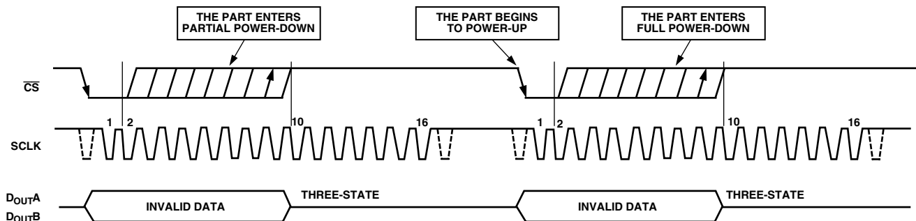
Figure 19. Entering Full Power-Down Mode
