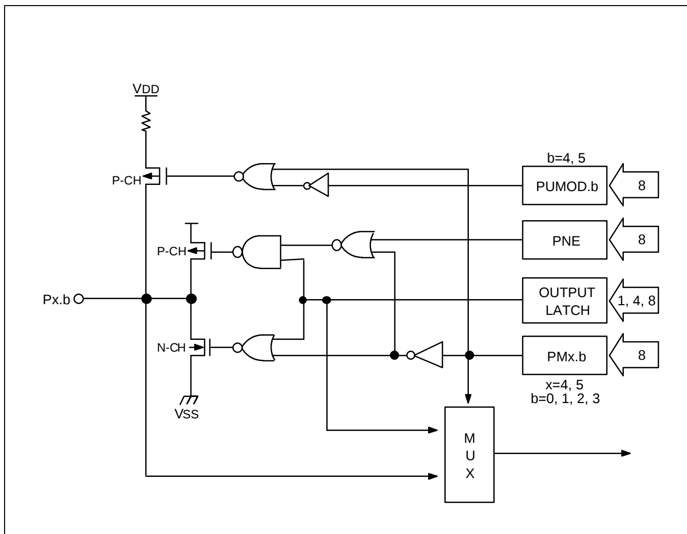
Figure 10-5. Circuit Diagram for Ports 4 and 5
