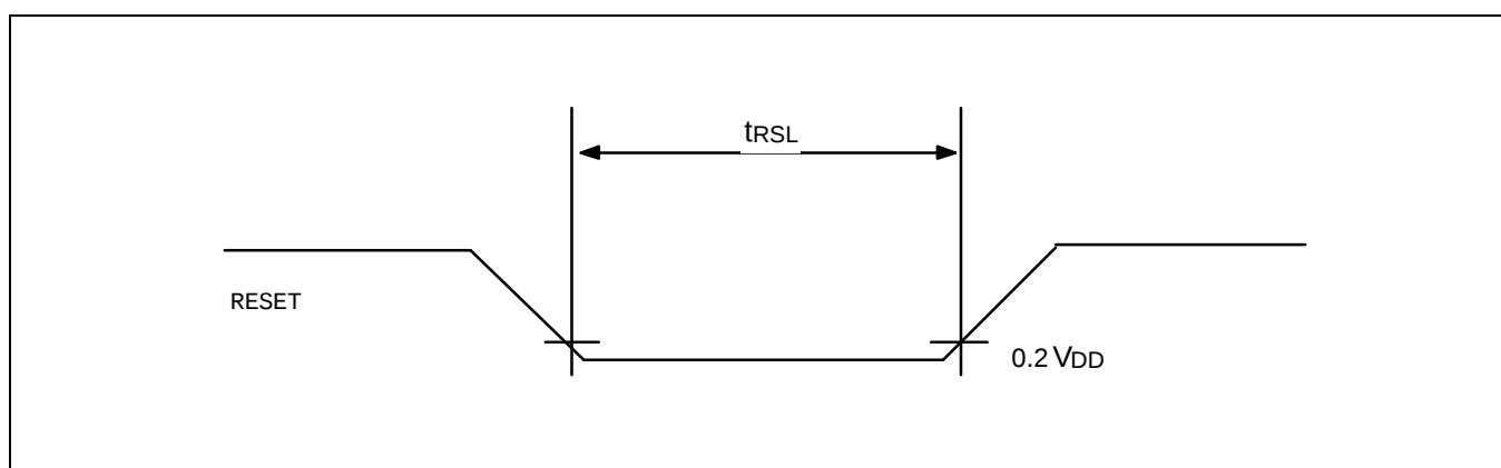
Figure 14-7. Input Timing for RESET Signal
