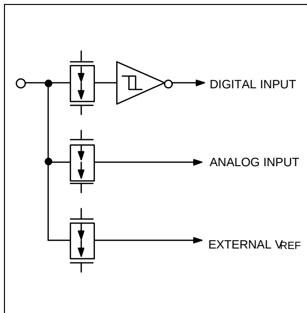
Figure 1-10. Pin Circuit Type F-2
