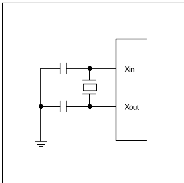
Figure 6–2. Crystal/Ceramic Oscillator
