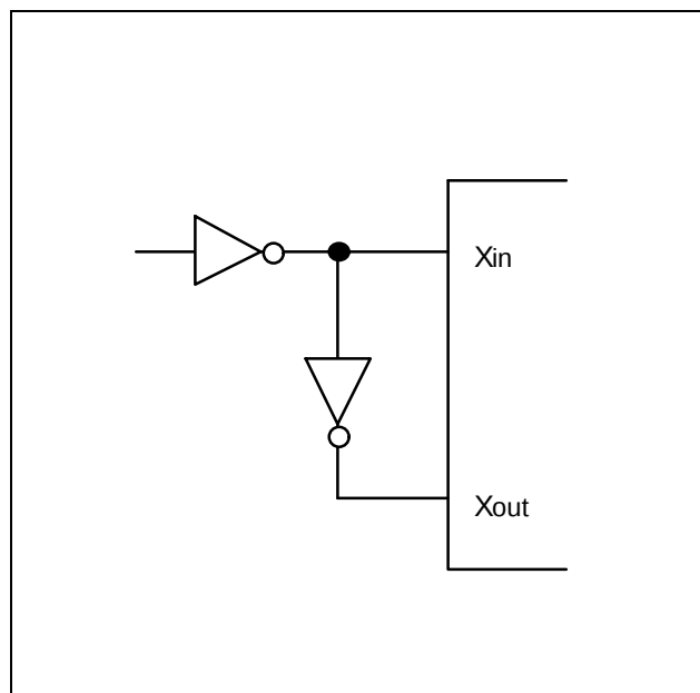
Figure 6–3. External Clock
