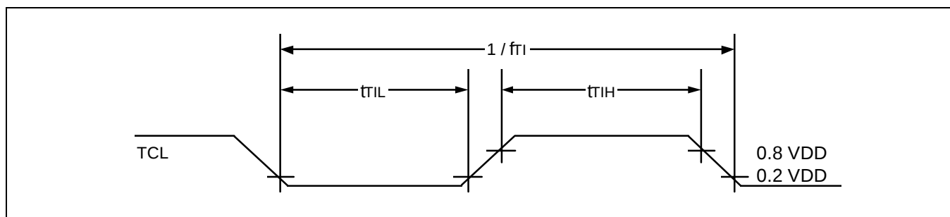
Figure 14-6. TCL Timing
