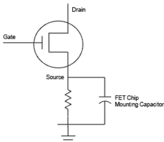
Figure 2. Schematic Diagram
