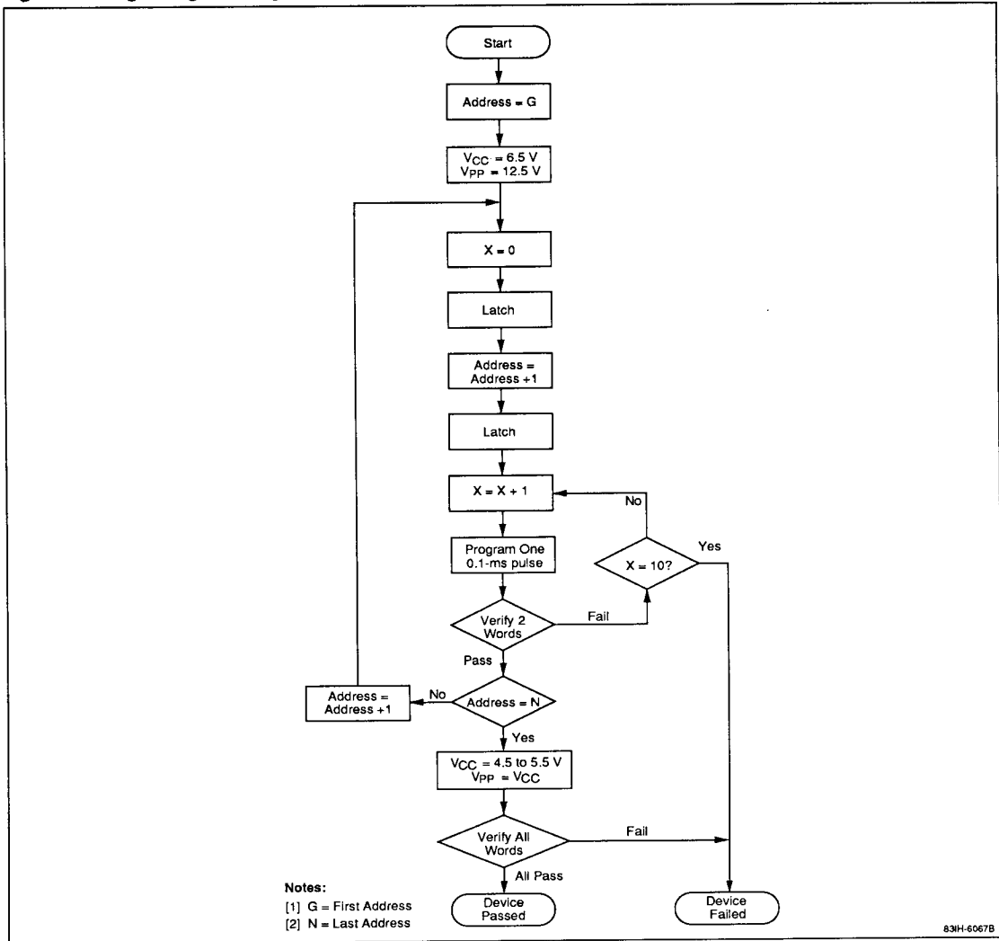
Figure 2. Page Programming Flowchart
