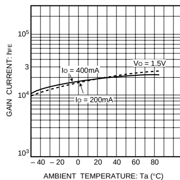
Fig.7 DC current amplification ratio vs. ambient temperature (I) (when Vo = 1.5V)
