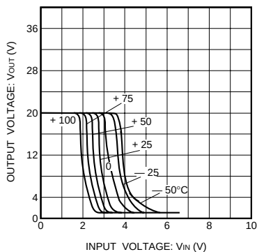
Fig.5 Output voltage vs. input voltage (temperature characteristic)
