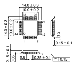
QFP44
