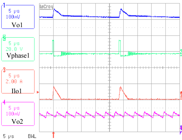
FIGURE 17. OPERATION AT LIGHT LOAD OF 100 MA, CHANNEL 1
