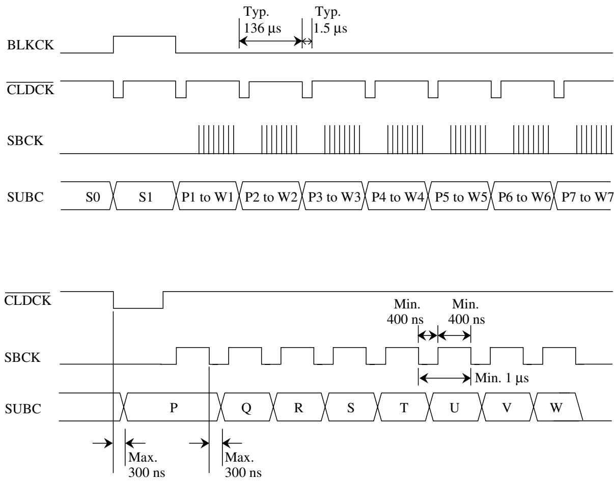
Figure 7-2-6 CLDCK, SUBC and SBCK timing
