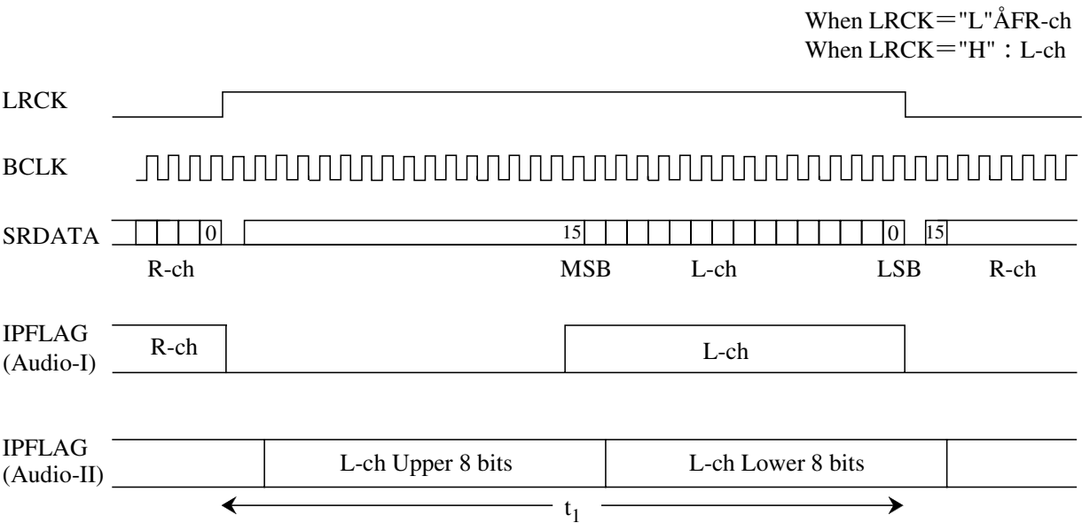
Figure 7-2-1 LRCK, BCLK, SRDATA and IPFLAG output timing
