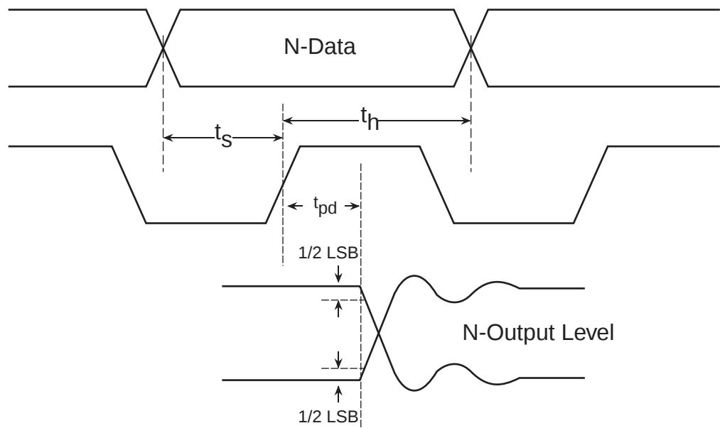
Figure 1 – Timing Diagram
