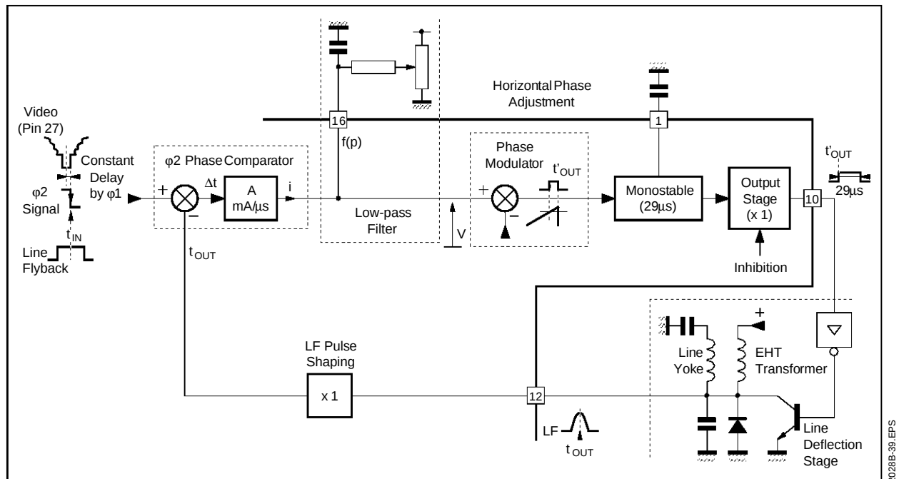
Figure 36 : Second Phase Locked Loop " \phi_2 " Block Diagram
