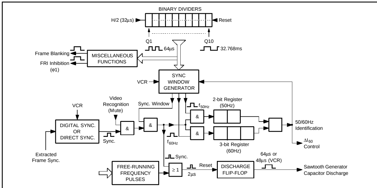
Figure 56 : Block Diagram
