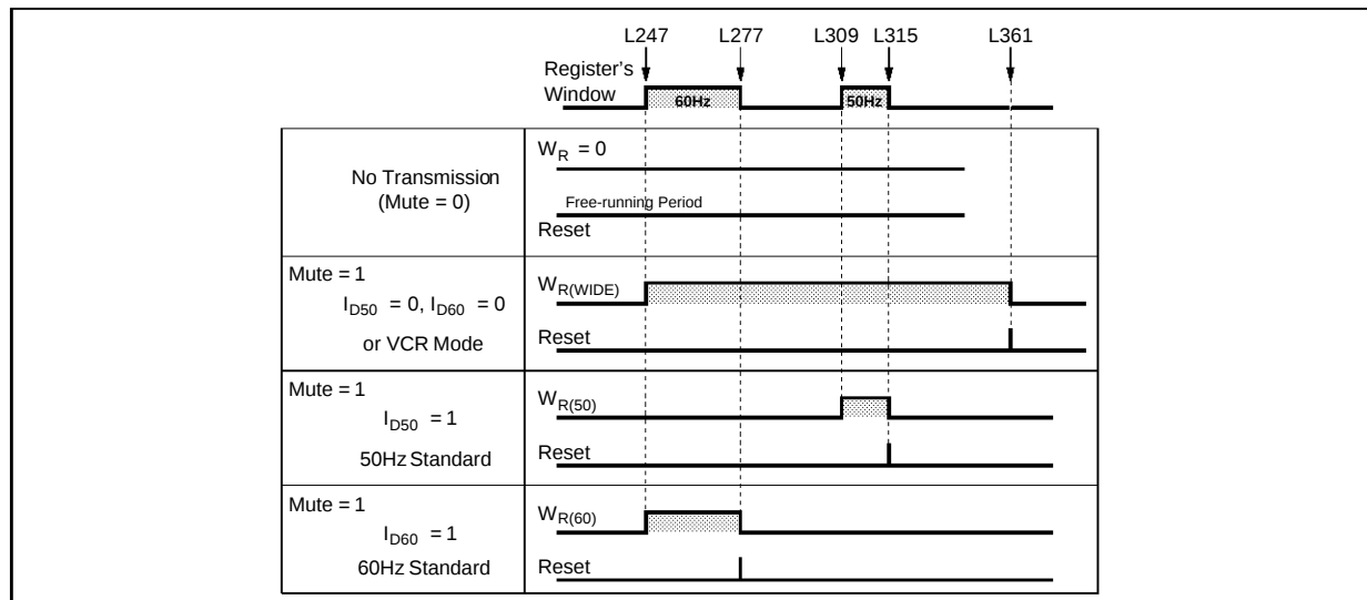
Figure 58 : Definition of Synchronization Windows and Free-running Periods
