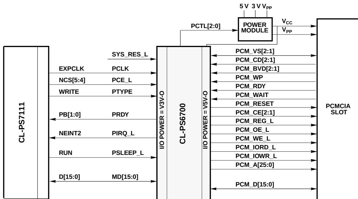
Figure 3-5. CL-PS7111-to-CL-PS6700 Interface
