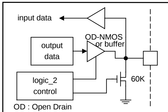
Input/Output IOB port : IOB2 - 0
