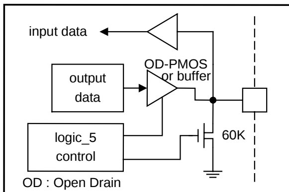
Input/Output IOD port : IOD3 - 0
