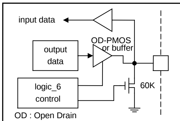
Input/Output IOD port : IOD7 - 4
