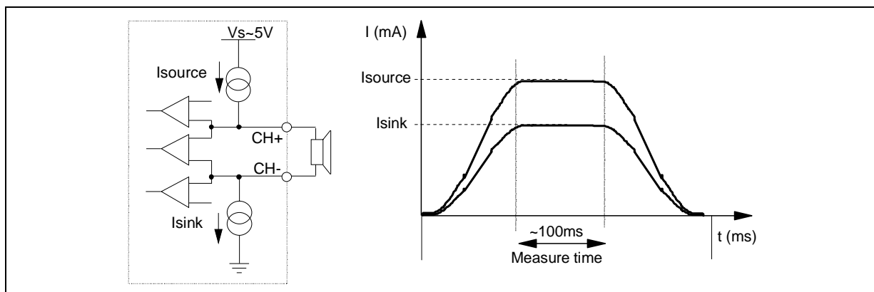
Fig. 15 and 16 show SVR and OUTPUT waveforms at the turn-on (stand-by out) with and without TURN-ON DIAGNOSTIC.
