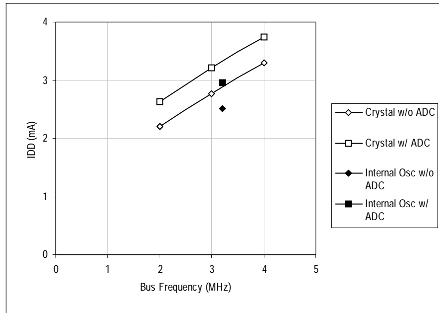
Figure 19-8. Typical 3-Volt Run Current versus Bus Frequency (25°C)
