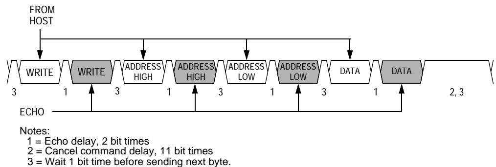
Figure 9-8. Write Transaction
