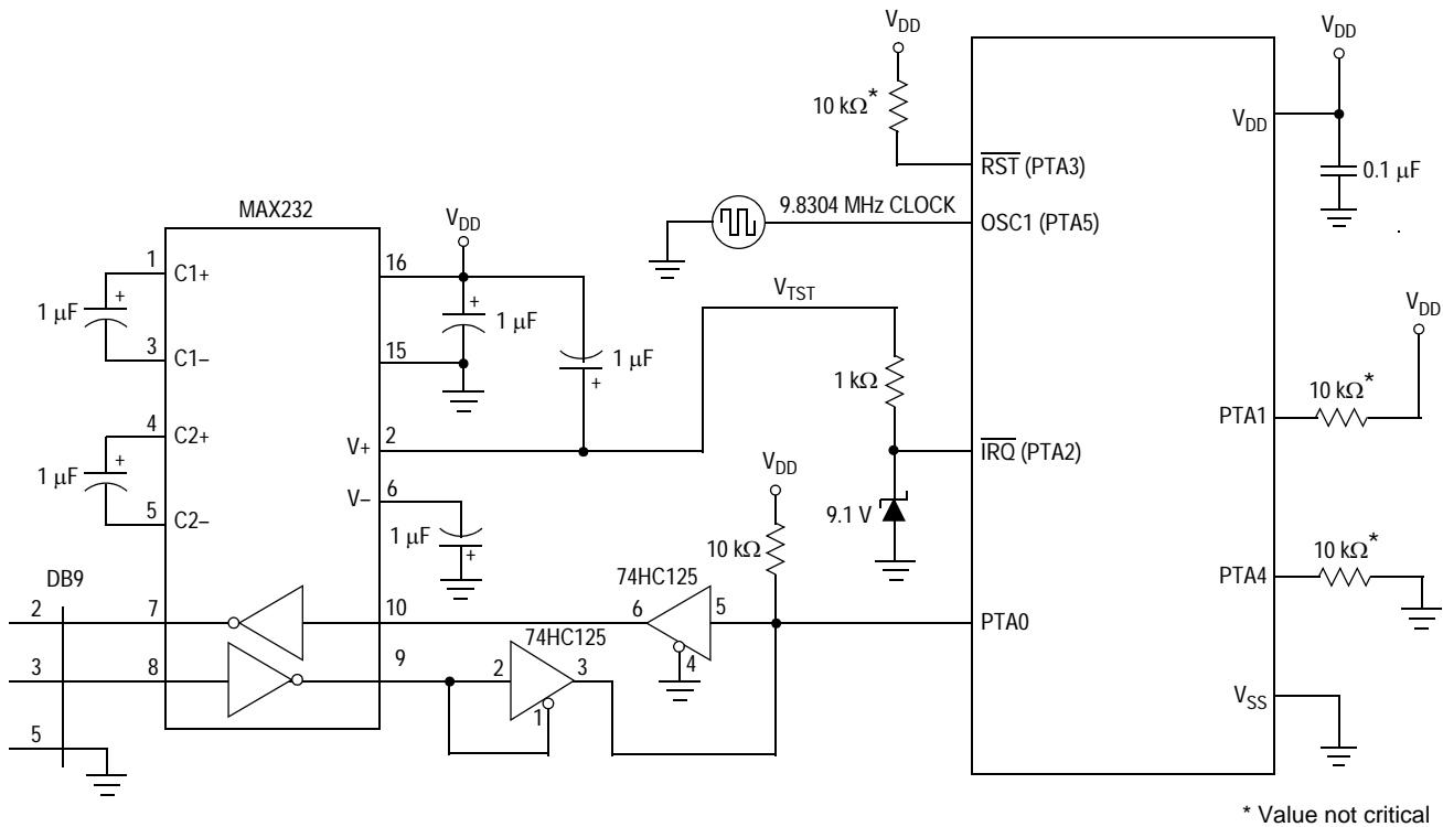
Figure 9-3. Monitor Mode Circuit (External Clock, with High Voltage)
