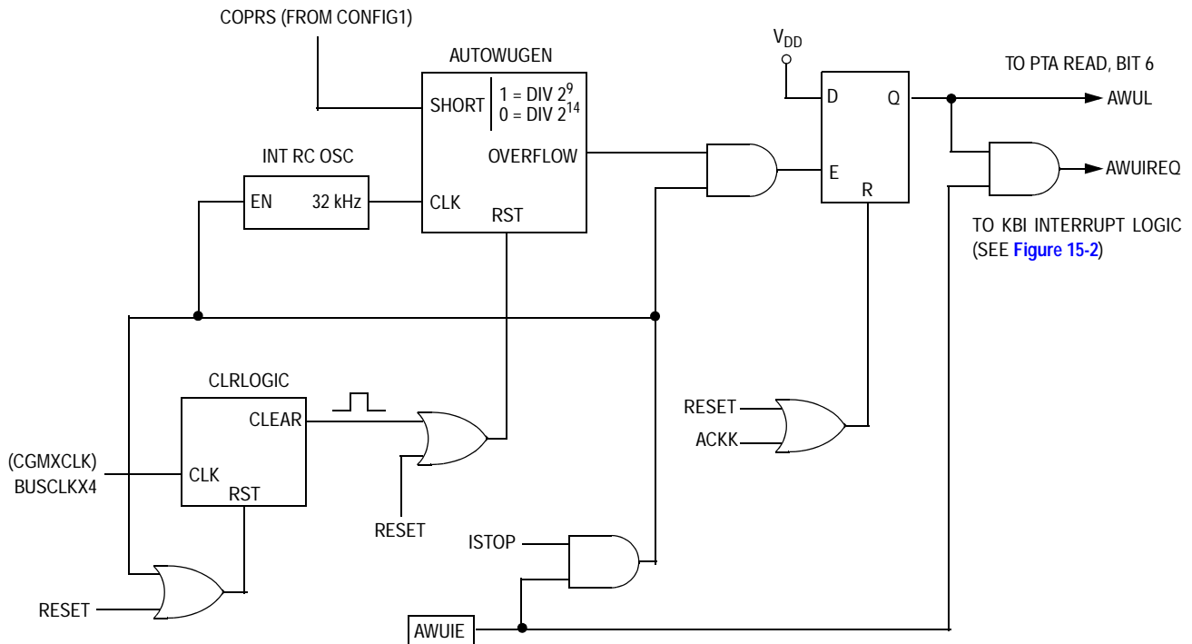
Figure 15-2. Auto Wakeup Interrupt Request Generation Logic
