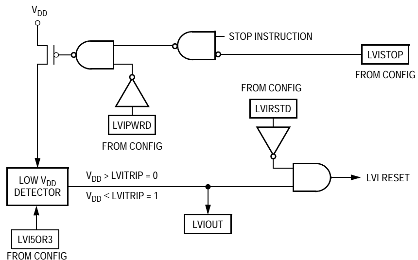
Figure 17-1. LVI Module Block Diagram
