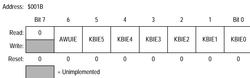
Figure 15-5. Keyboard Interrupt Enable Register (KBIER)
