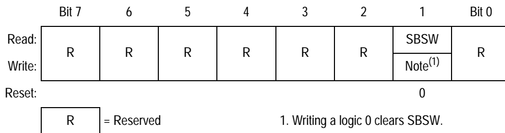
Figure 18-7. Break Status Register (BSR)
