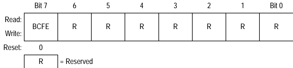
Figure 18-8. Break Flag Control Register (BF CR)
