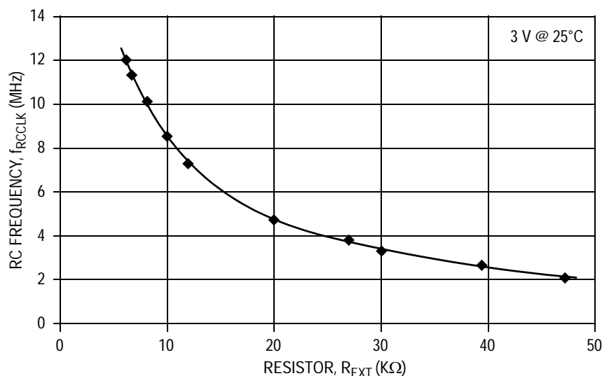
Figure 19-6. RC versus Frequency (3 Volts @ 25°C)
