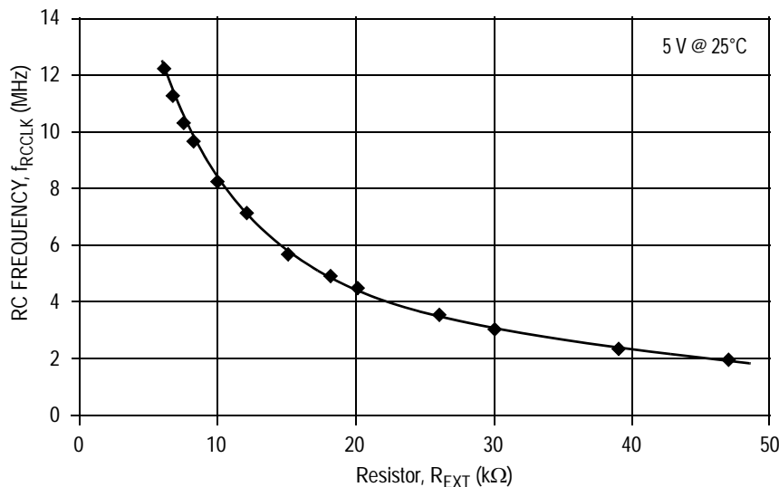
Figure 19-3. RC versus Frequency (5 Volts @ 25°C)
