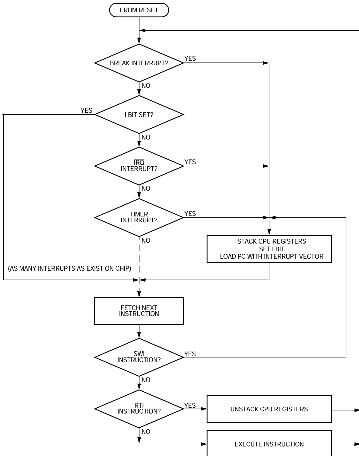
Figure 7-8. Interrupt Processing
