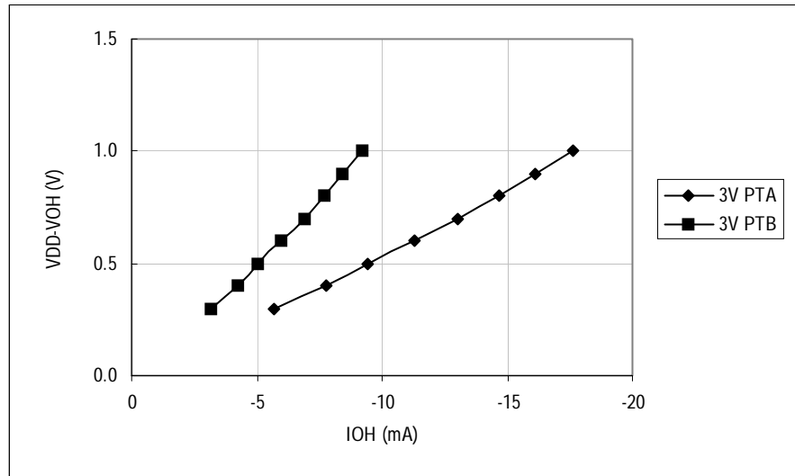
Figure 19-4. Typical 3-Volt Output High Voltage versus Output High Current (25°C)
