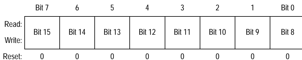
Figure 18-4. Break Address Register High (BRKH)
