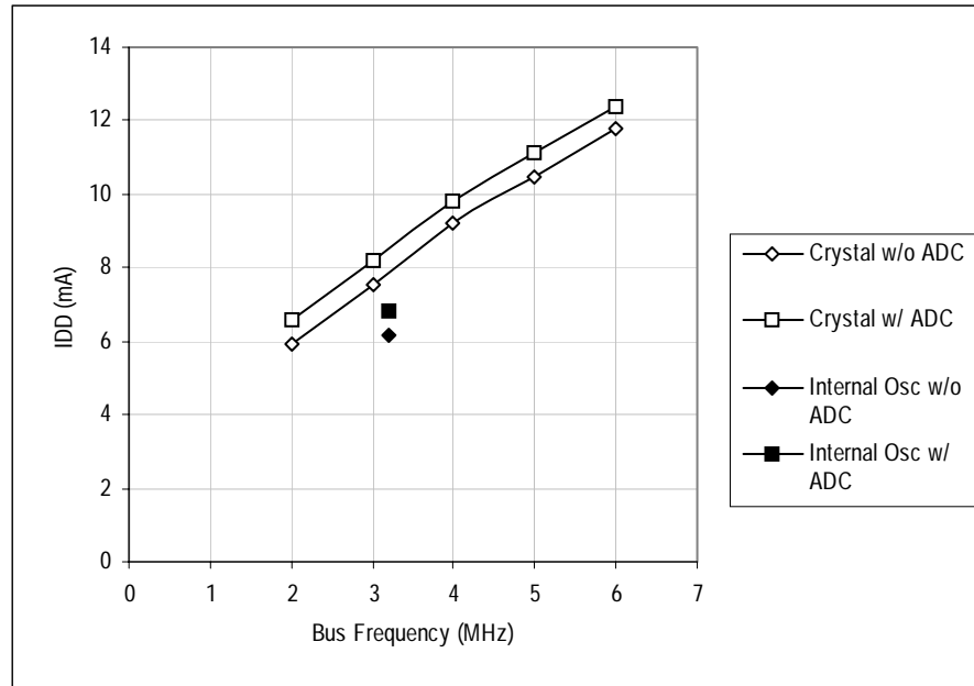
Figure 19-7. Typical 5-Volt Run Current versus Bus Frequency (25°C)
