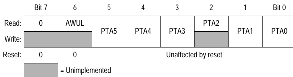
Figure 15-3. Port A Data Register (PTA)
