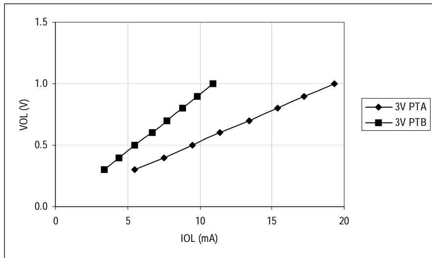
Figure 19-5. Typical 3-Volt Output Low Voltage versus Output Low Current (25°C)
