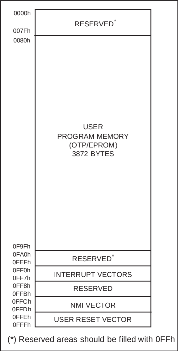
Figure 4. ST62E45B/T45B Program Memory Map
