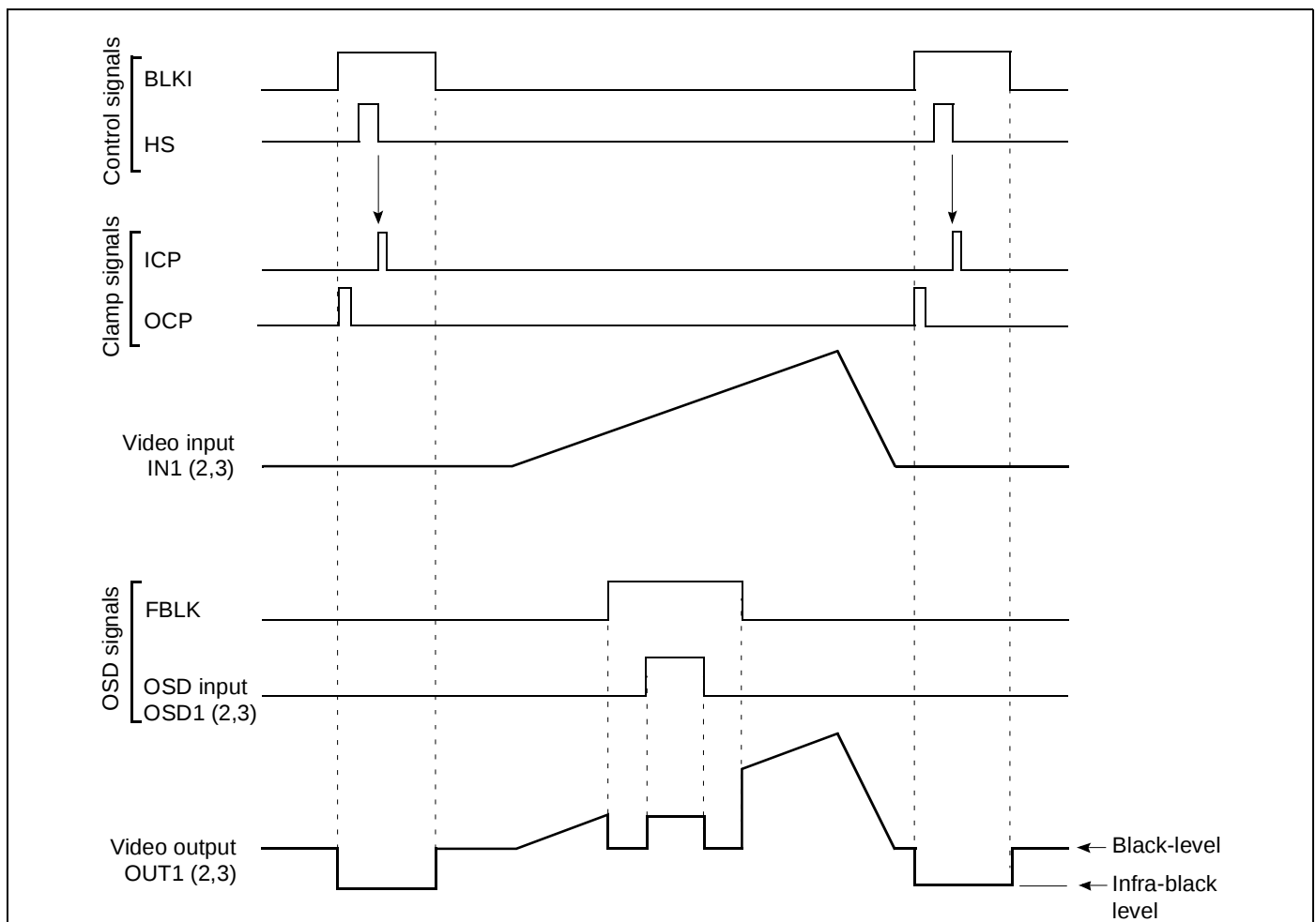
Figure 18: Signal Waveforms
