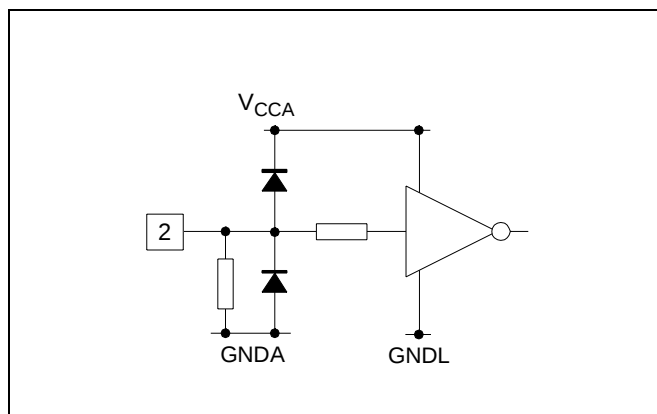
Figure 25: Hsync Input
