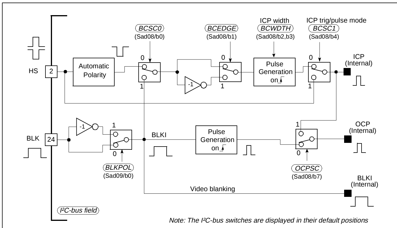
Figure 3: ICP, OCP and BLKI Generation
