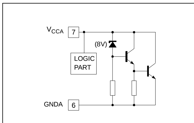
Figure 27: Analog Supplies
