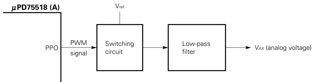
Fig. 4-33 Sample Configuration of D/A Conversion Using μPD75518(A)
