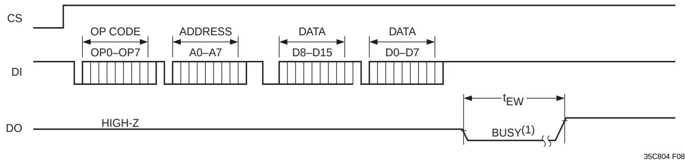
Figure 5. Program/Erase Timing (x16 Format)
