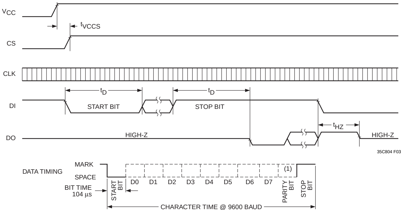
Figure 1. A.C. Timing
