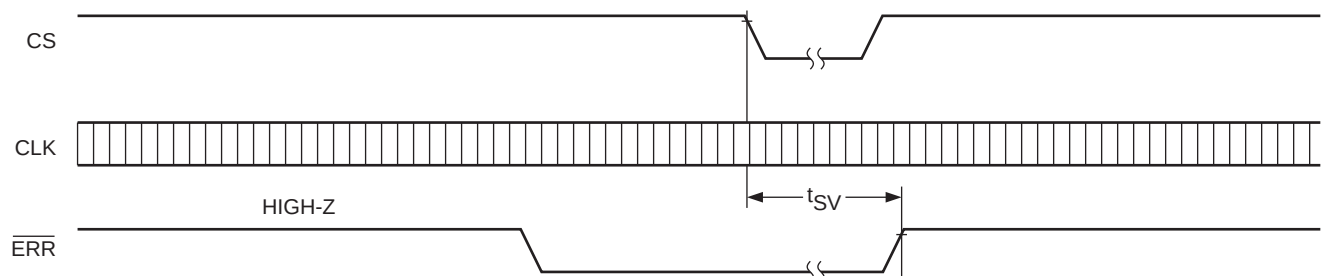
Figure 10. \overline{\text{ERR}} Pin Timing
