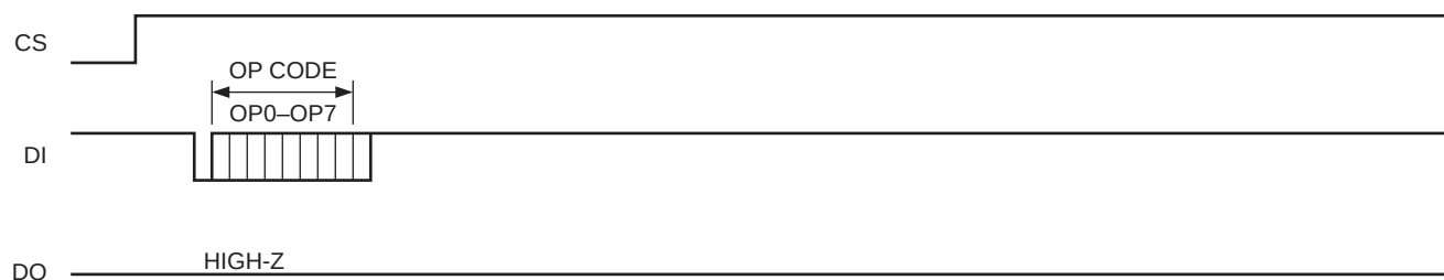
Figure 9. EWEN/EWDS Timing (x16 Format)
