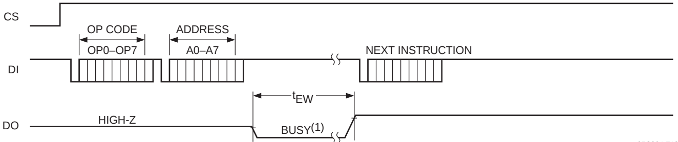
Figure 12. Erase Timing (x16 Format)
