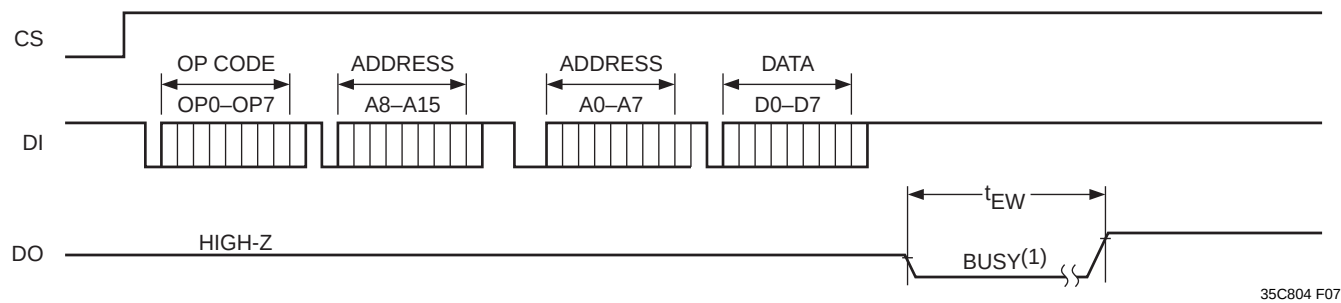
Figure 4. Program/Erase Timing (x8 Format)
