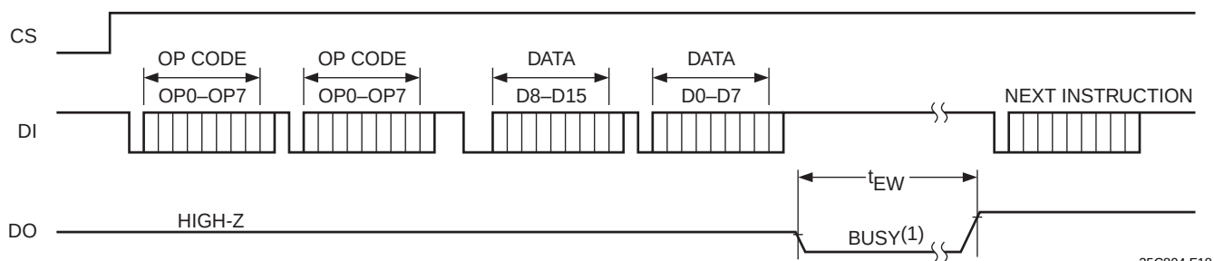
Figure 17. WRAL Timing (x16 Format)
