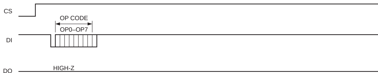
Figure 8. EWEN/EWDS Timing (x8 Format)
