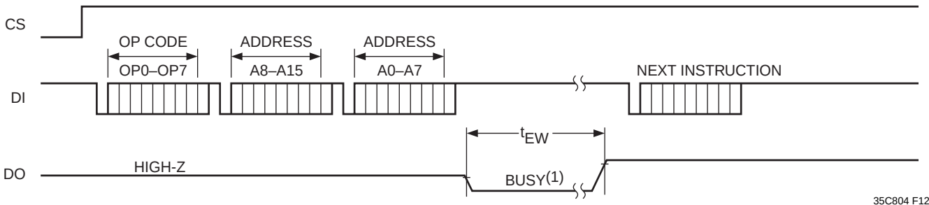
Figure 11. Erase Timing (x8 Format)
