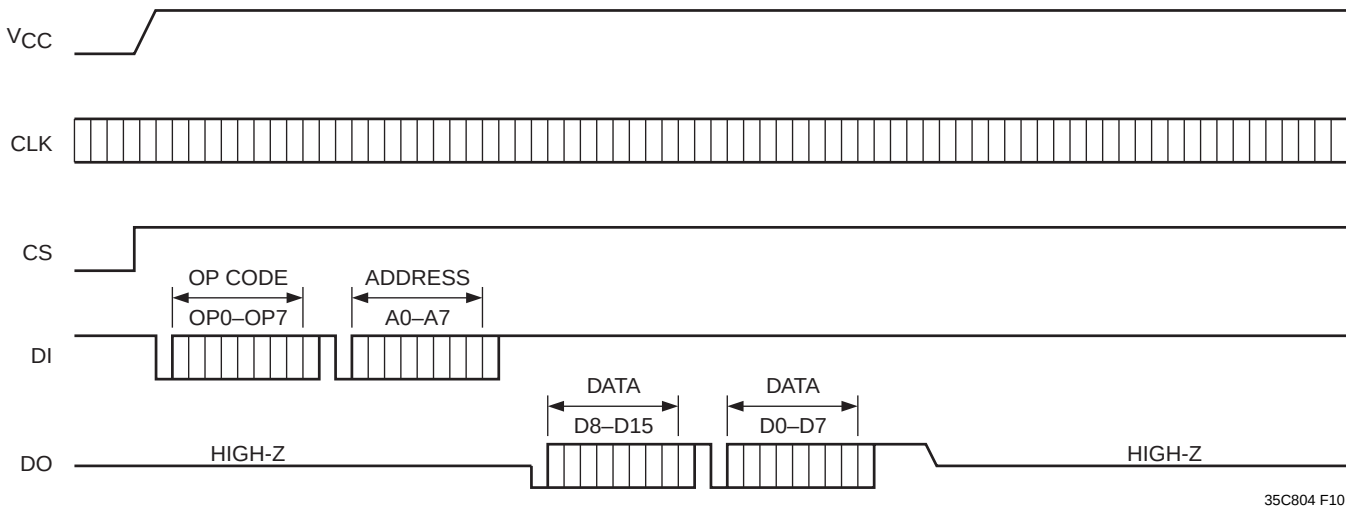
Figure 7. Read Timing (x16 Format)
