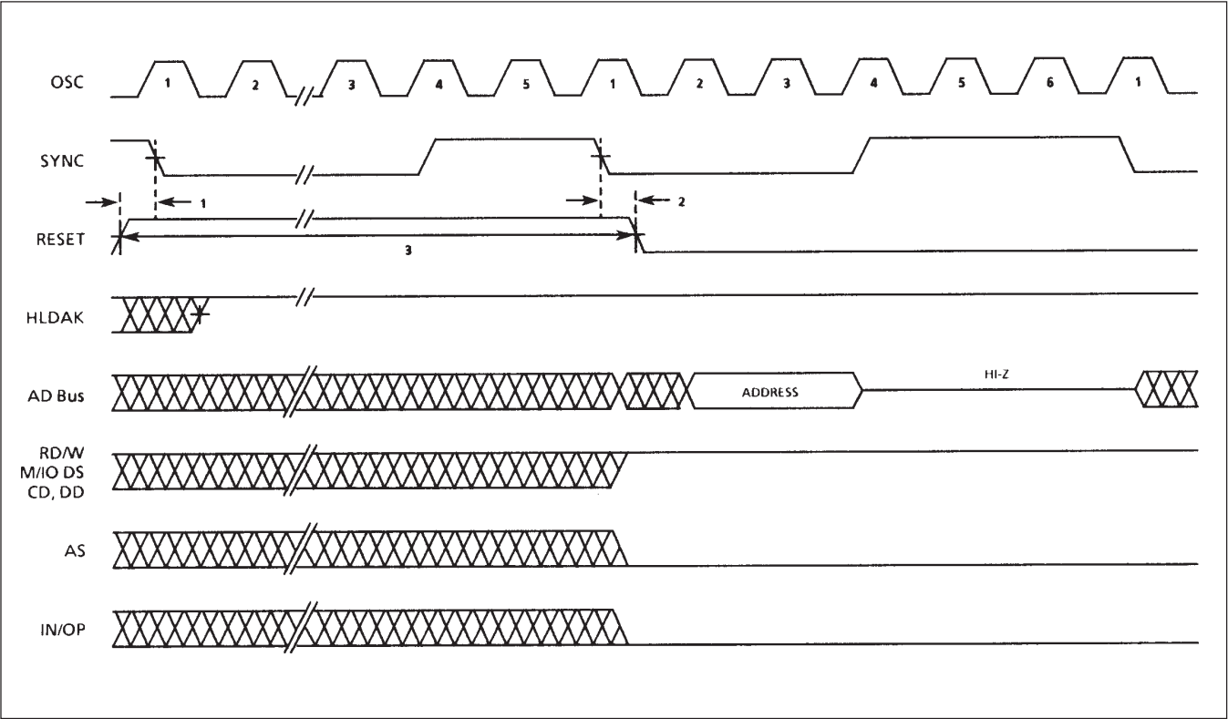
Figure 12: Reset Timing
