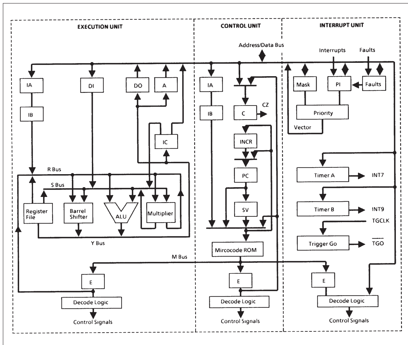
Figure 2: MAS281 Architecture
