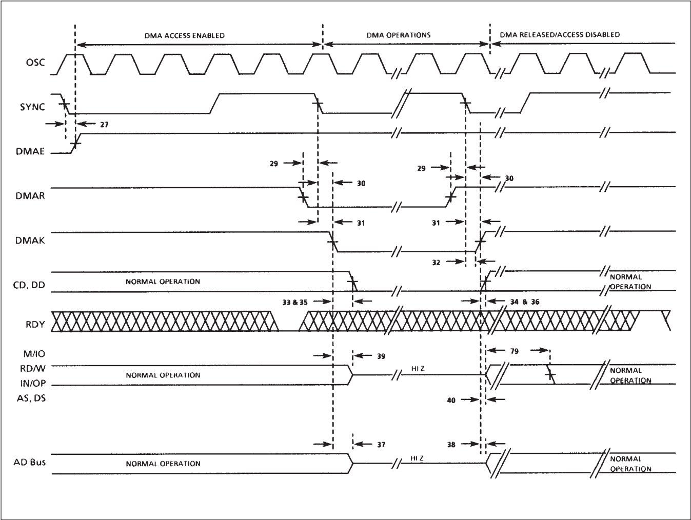
NOTE: Other required input states: DTIMER = HIGH and RESET = LOW Figure 18: DMA Access/Release Timing
