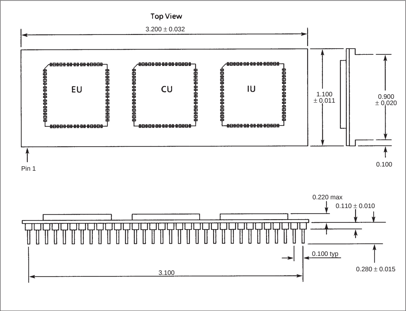
Figure 27: Dimensioned Drawing
