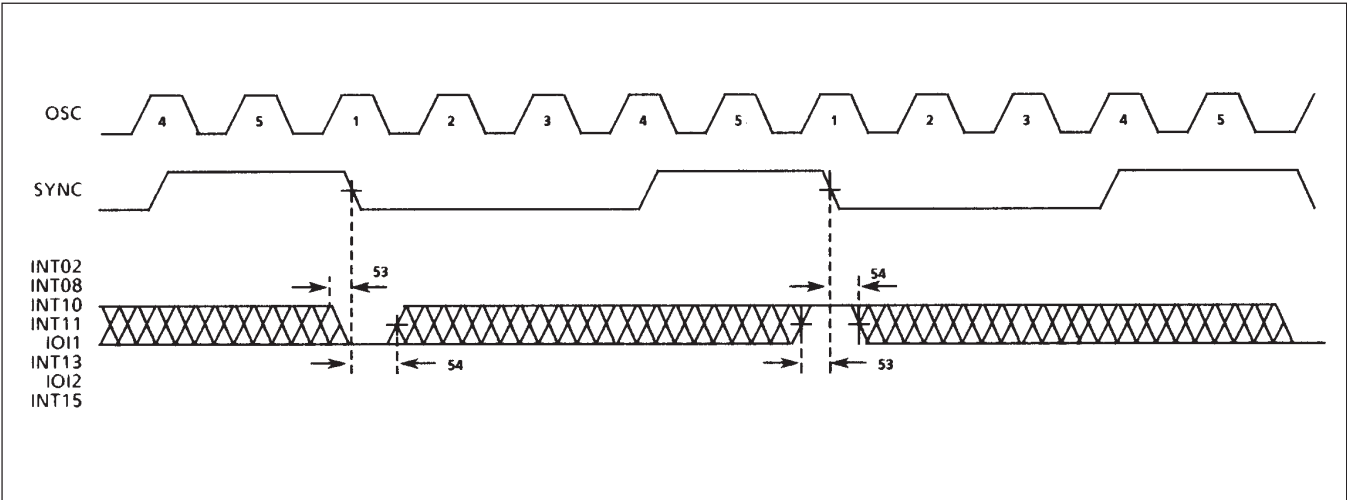
NOTE: Other required input: RESET = LOW Figure 19: Interrupt Request Timing
