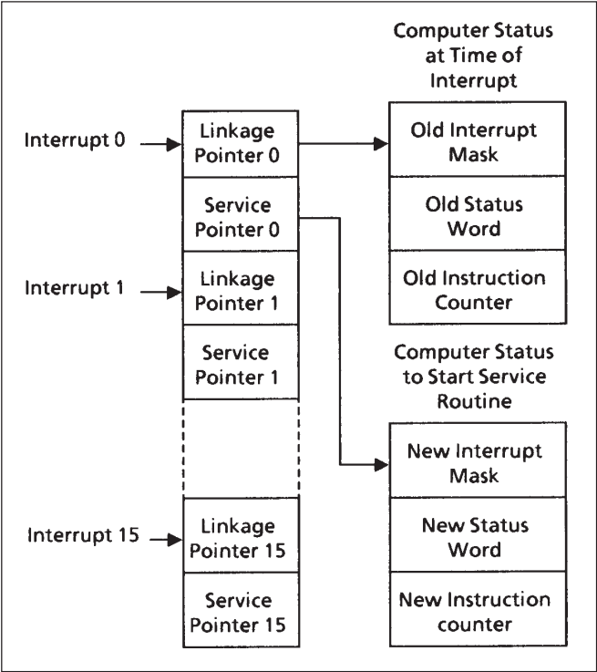
Figure 6: Interrupt Vectoring
