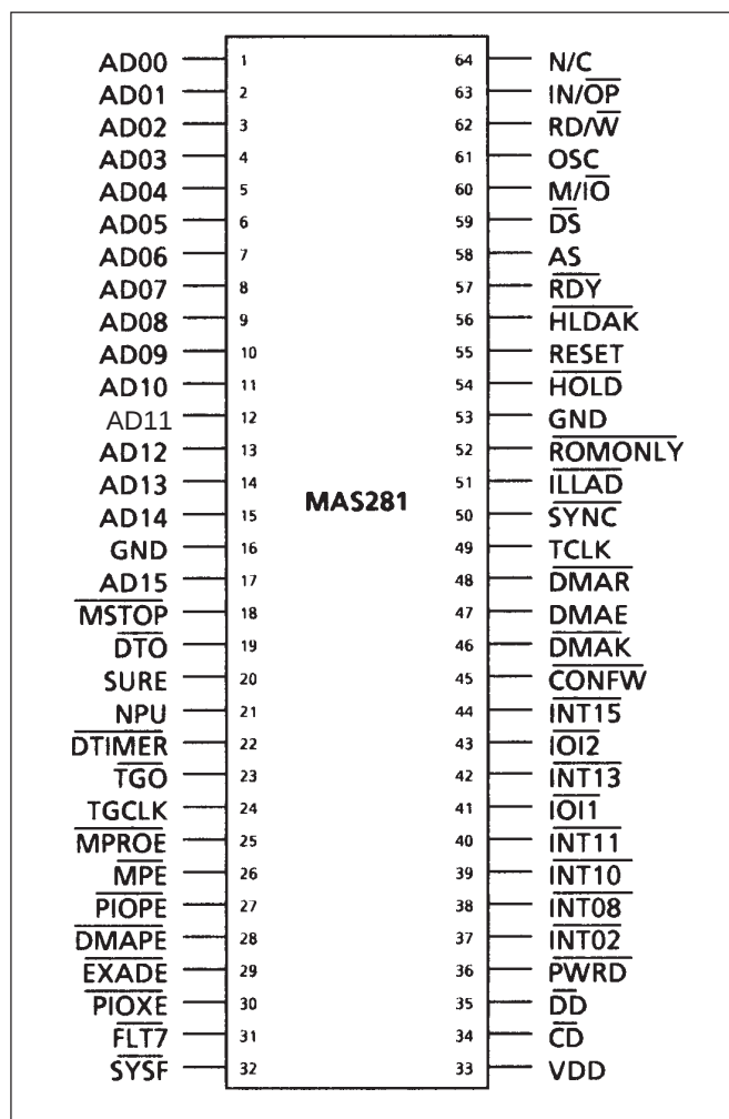
Figure 4: Pin Assignments
