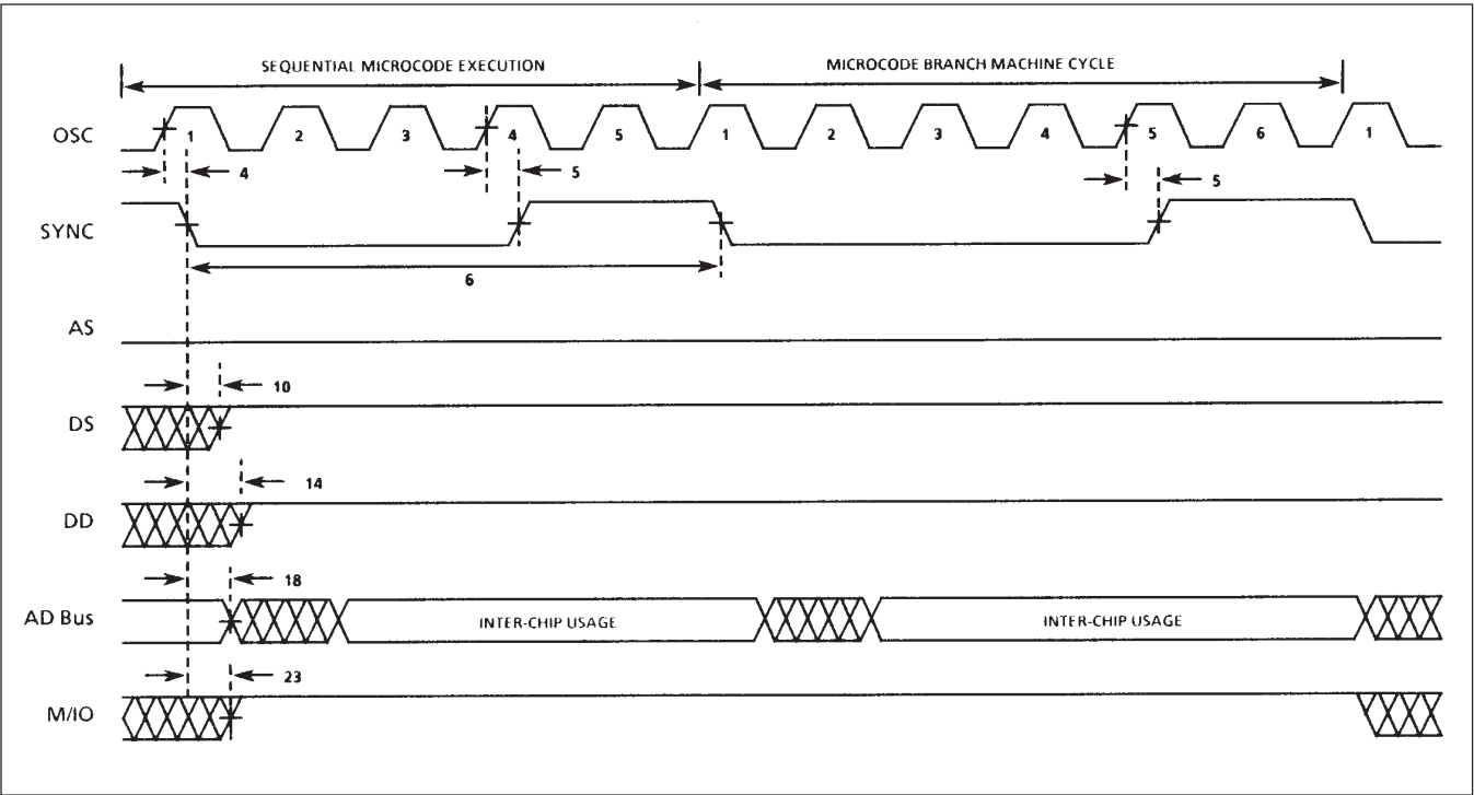
Figure 13: Internal CPU Operations
