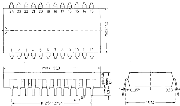
Fig. 8: SAA 1250 in 24-pin DII Plastic Package, 20 B 24 according to DIN 41 866
