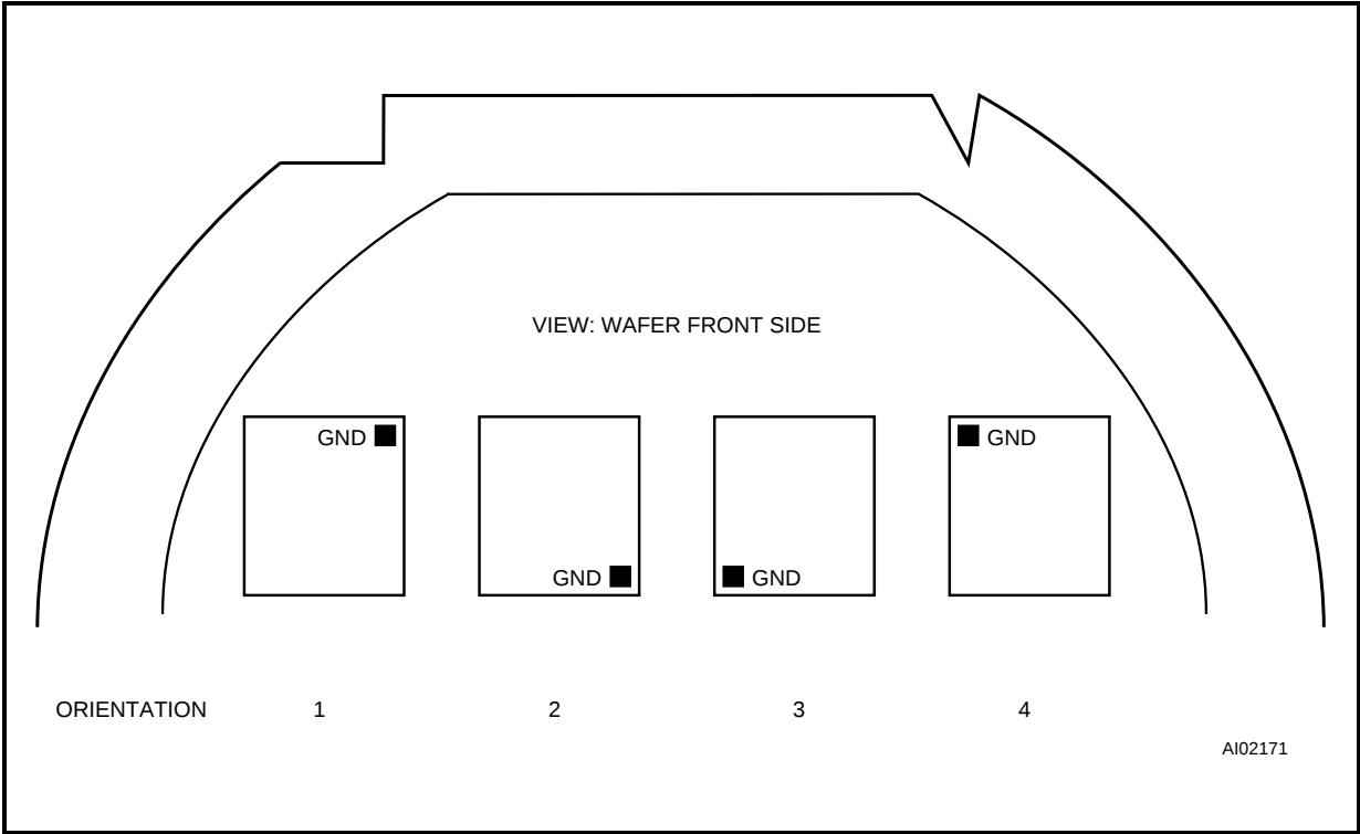
Figure 2. Sawing orientation
