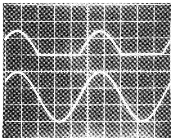
FIGURE 9B. OUTPUT WAVEFORM WITH GROUND REFERENCE SINE-WAVE INPUT
