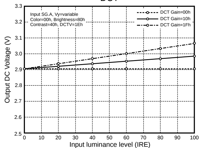
DCT
