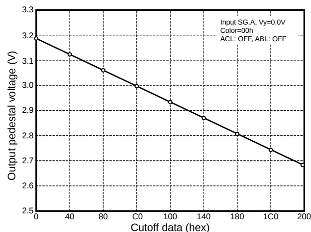
Cutoff control
