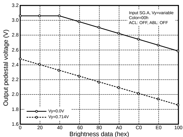
Brightness control
