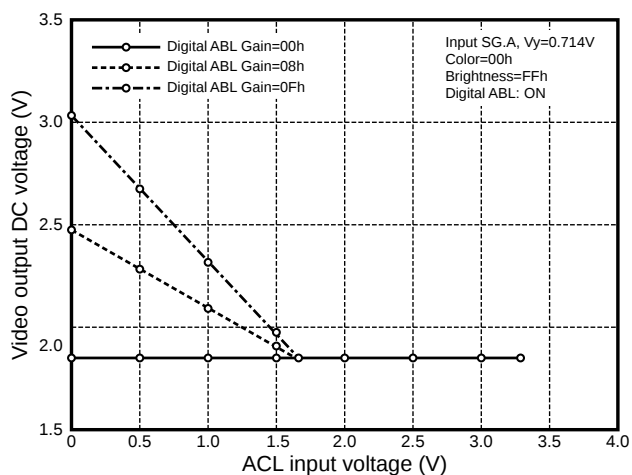
ABL characteristic
