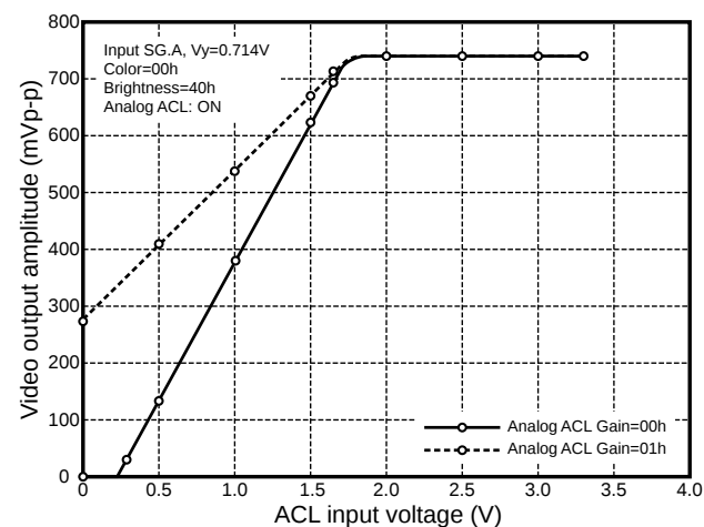
ACL characteristic
