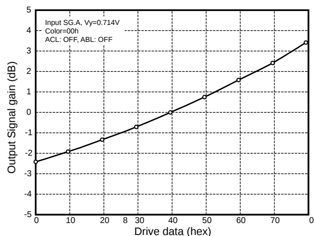
Drive control
