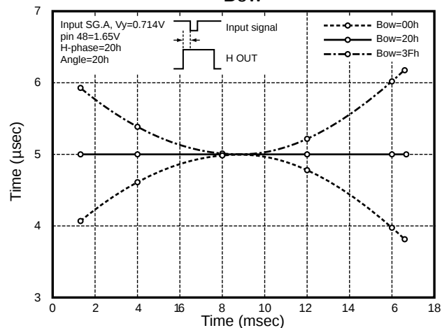
Bow
