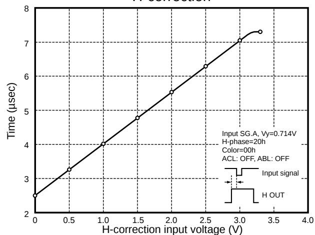
H-correction
