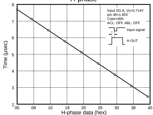
H-phase
