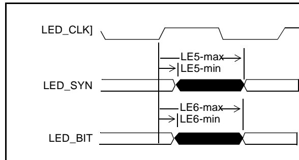
Figure 18 - AC Characteristics – LED Interface
