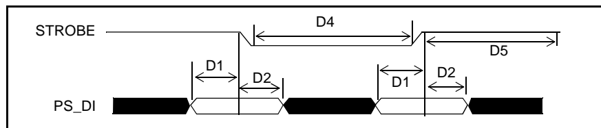
Figure 23 - Serial Interface Setup Timing
