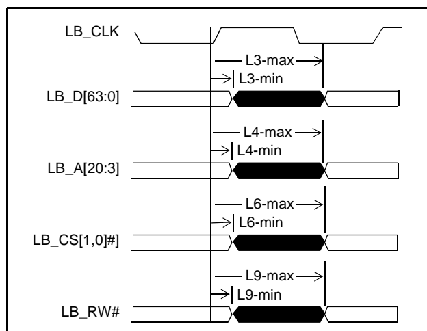
Figure 9 - Local Memory Interface - Output valid delay timing
