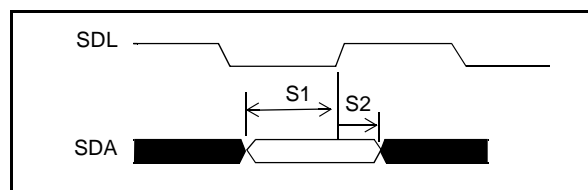
Figure 21 - I 2 C Input Setup Timing
