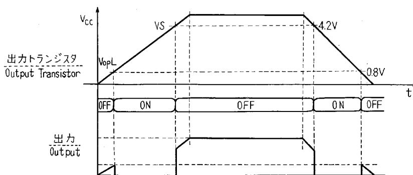
[Fig. 1] PST519 の動作/Operation of PST519
