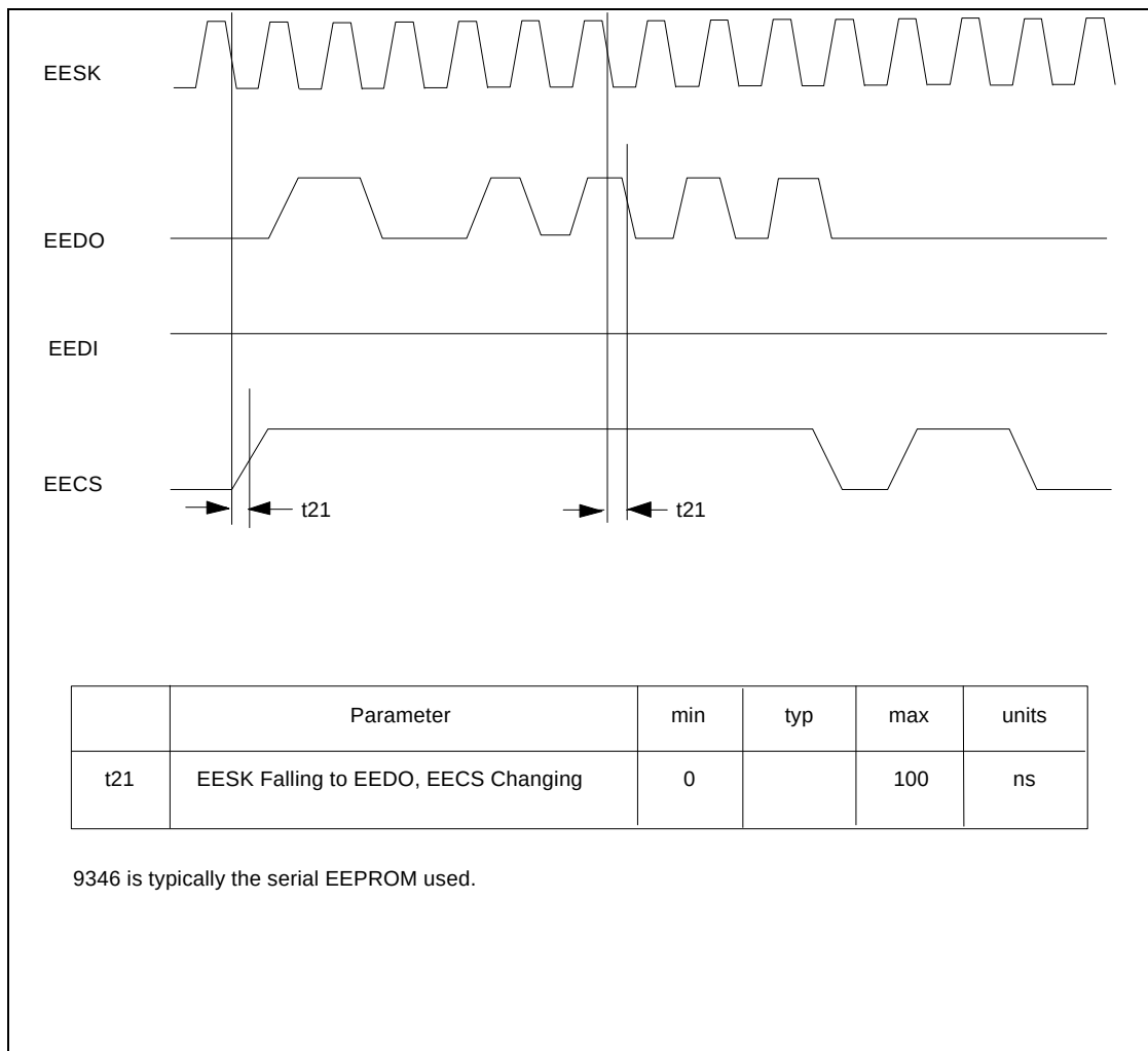
FIGURE 36 - EEPROM READ
