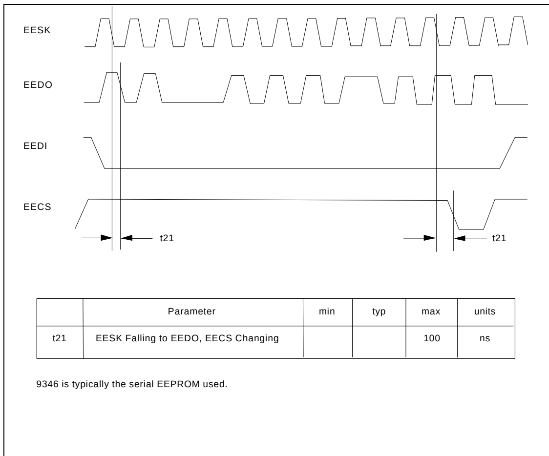
FIGURE 37 - EEPROM WRITE
