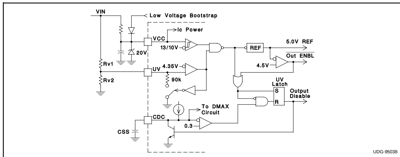
Figure 1: Undervoltage Lockout
