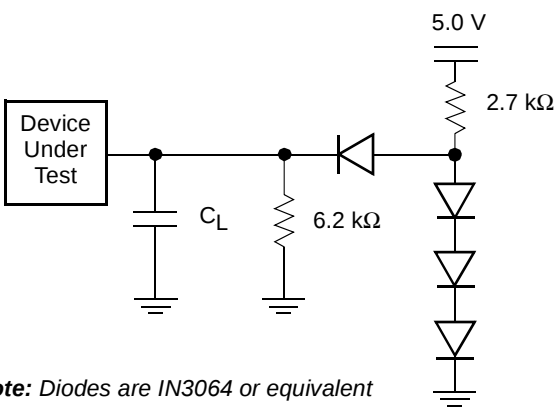
Figure 8. Test Setup
