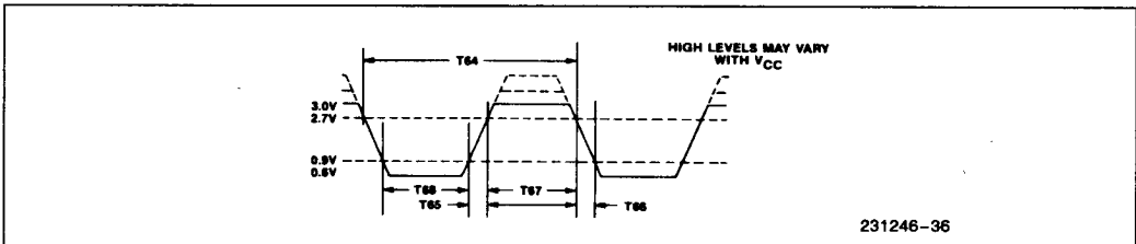
Figure 35. \overline{\text{RxC}} Input Voltage Levels for Timing Measurements *
