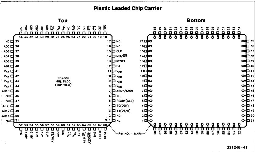
Figure 2. 82586 Pinout Diagrams
