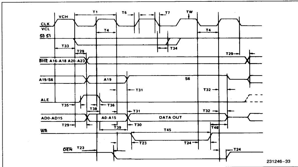
Figure 32. Write Cycle Timing
