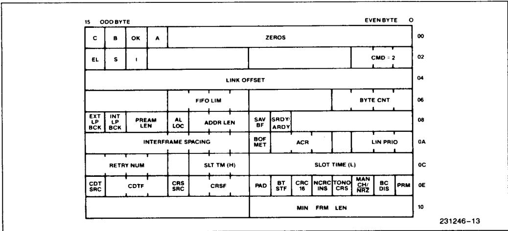
Figure 13. The CONFIGURE Command Block
