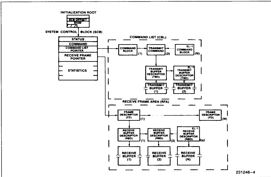
Figure 4. 82586 Shared Memory Structure
