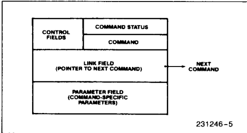
Figure 5. Action Command Format
