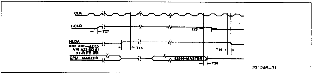
Figure 30. HOLD/HLDA Timing Relative to CLK
