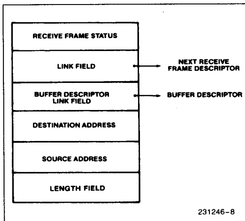
Figure 9. Receive Frame Descriptor
