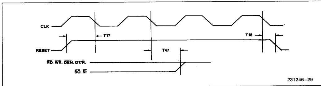
Figure 28. RESET Timing
