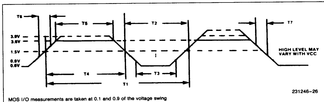
Figure 25. System Clock CMOS Input Voltage Levels for Timing Measurements
