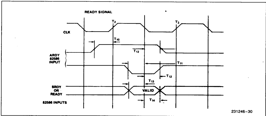
Figure 29. ARDY and SRDY Timings Relative to CLK
