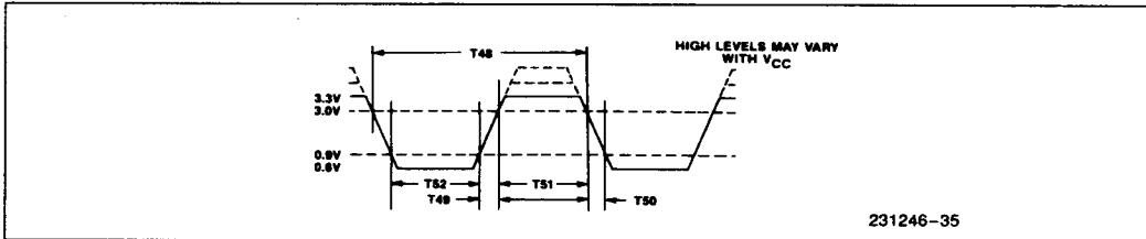
Figure 34. \overline{\text{TxC}} Input Voltage Levels for Timing Measurements
