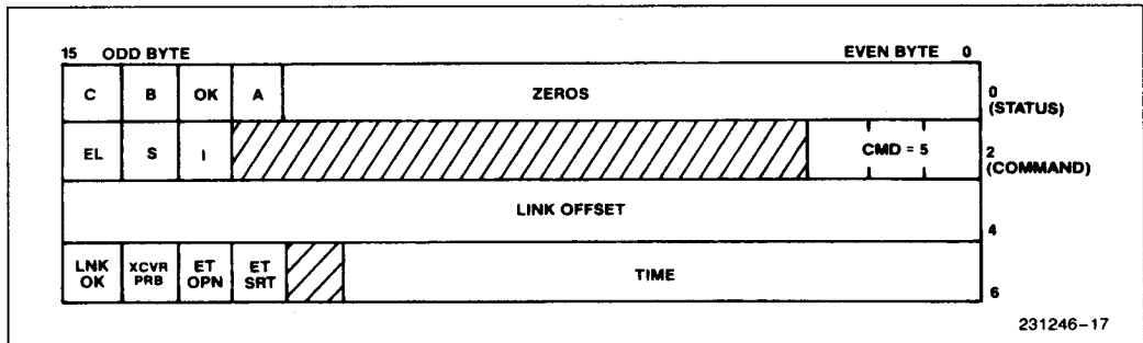
Figure 17. The TDR Command Block
