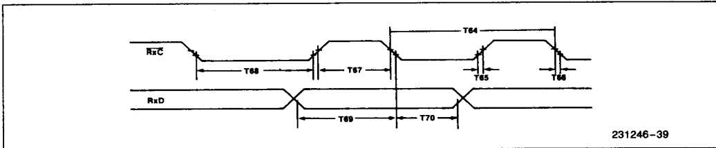
Figure 37. RxD Timing Relative to RxC
