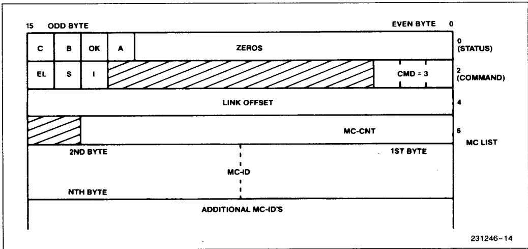
Figure 14. The MC-SETUP Command Block
