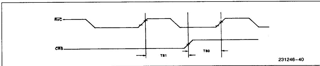
Figure 38. CRS Timing Relative to RxC
