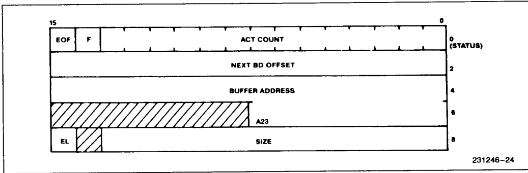
Figure 23. The Receive Buffer Descriptor (RBD) Format
