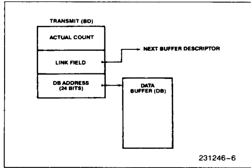
Figure 6. Data Buffer Descriptor and Data Buffer Structure
