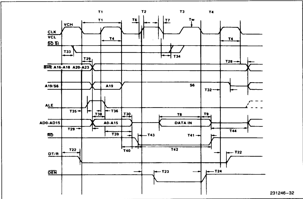
Figure 31. Read Cycle Timing
