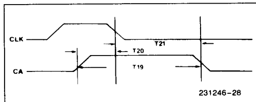
Figure 27. CA Input Timing
