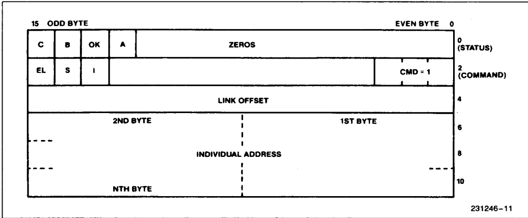
Figure 12. The IA-SETUP Command Block
