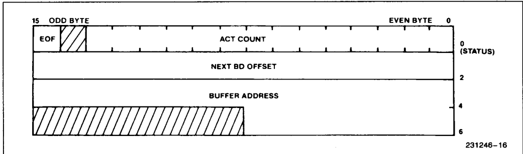
Figure 16. The Transmit Buffer Description
