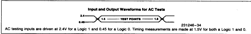
Figure 33. TTL Input/Output Voltage Levels for Timing Measurements
