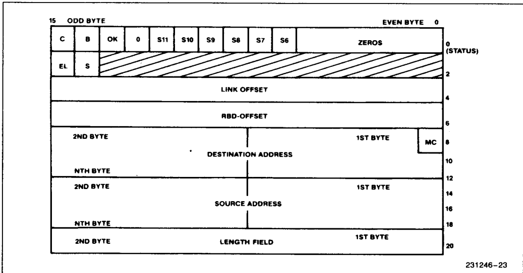
Figure 22. The Frame Descriptor (FD) Format
