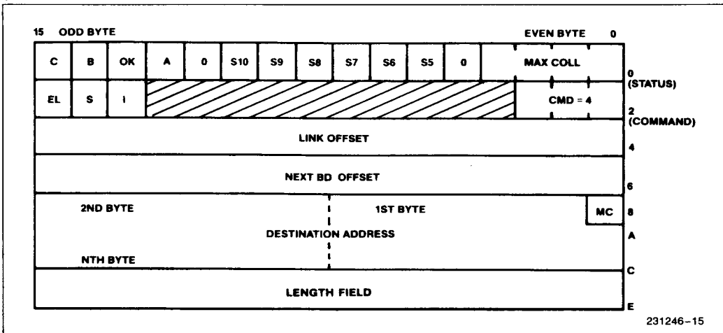
Figure 15. The Transmit Command Block
