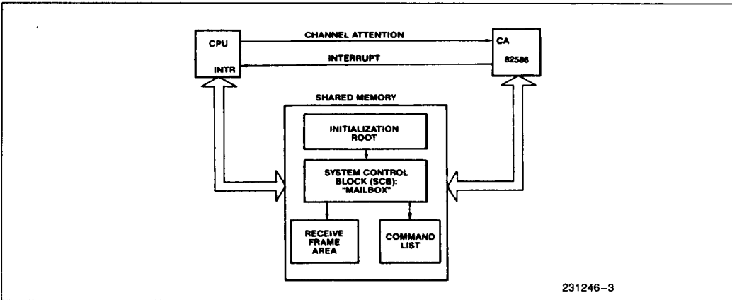
Figure 3. 82586/Host CPU Interaction
