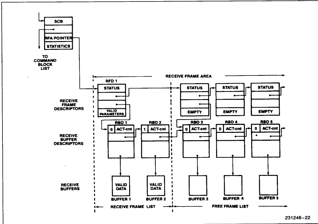
Figure 21. The Receive Frame Area
