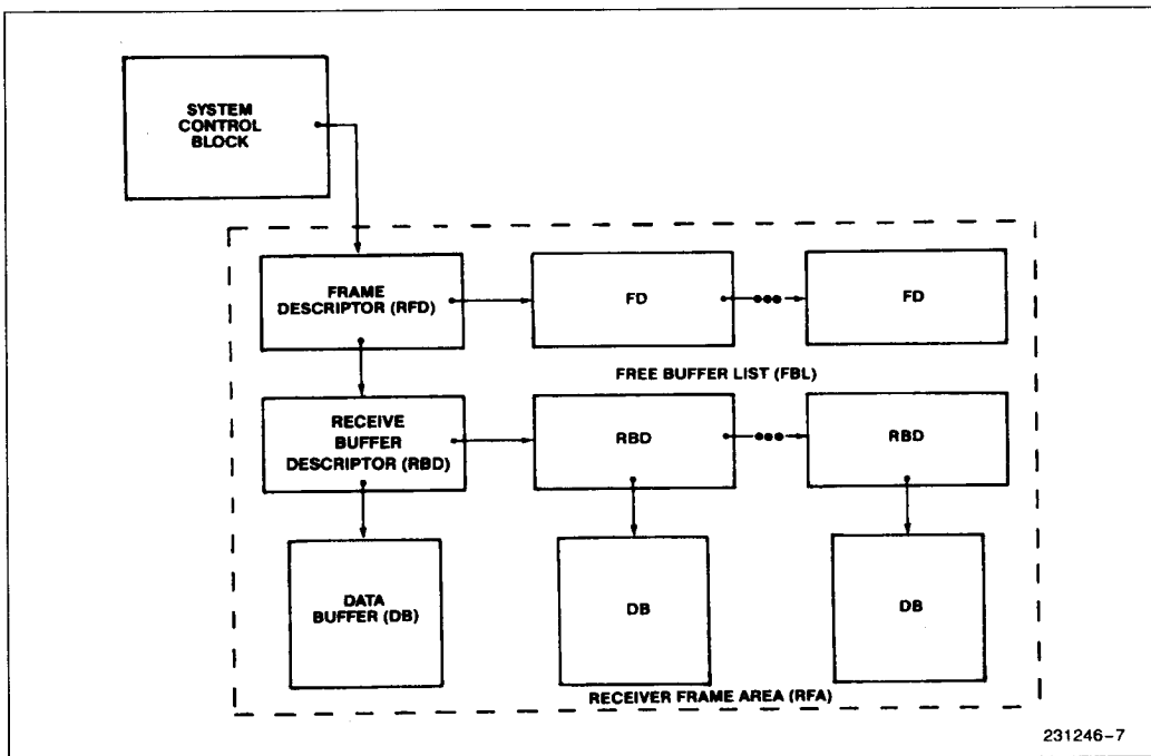
Figure 8. Receive Frame Area Diagram
