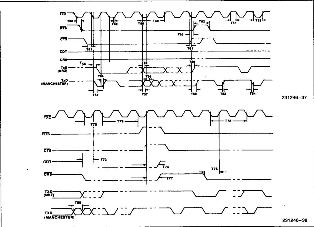
Figure 36. Transmit and Control and Data Timing
