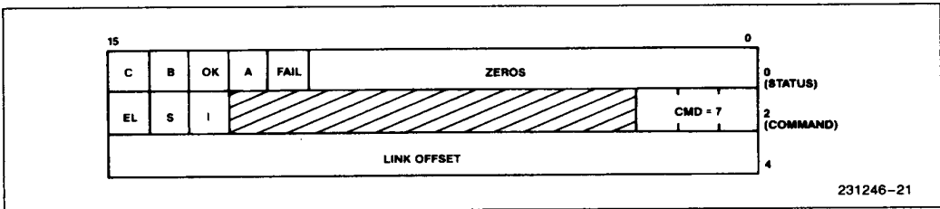
Figure 20. The DIAGNOSE Command Block
