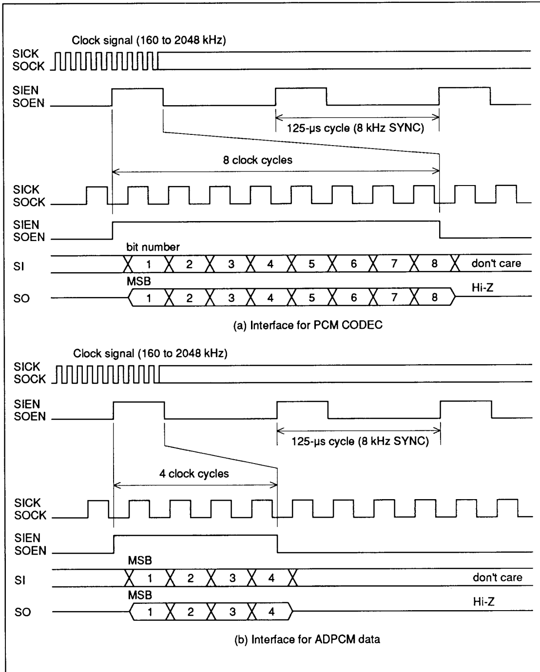
Figure 12 Serial Interface Timing
