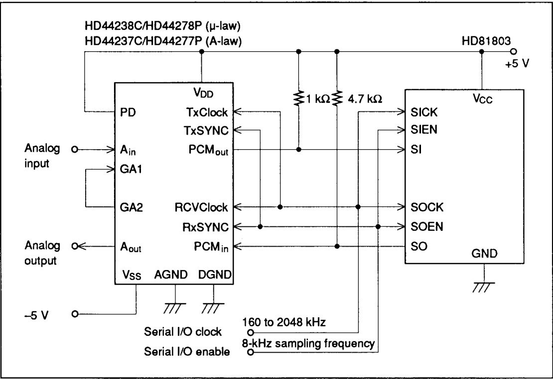
Figure 10 PCM CODEC Interface for the Parallel Mode
