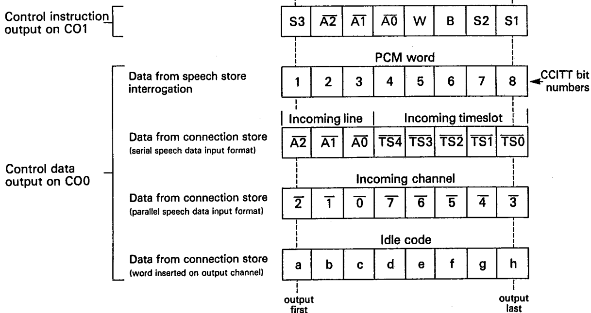
Figure 5. CONTROL INTERFACE OUTPUT MESSAGE FORMATS
