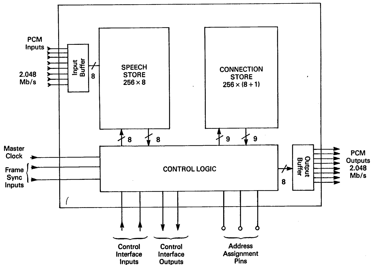
Fig. 1 DSM Block Diagram
