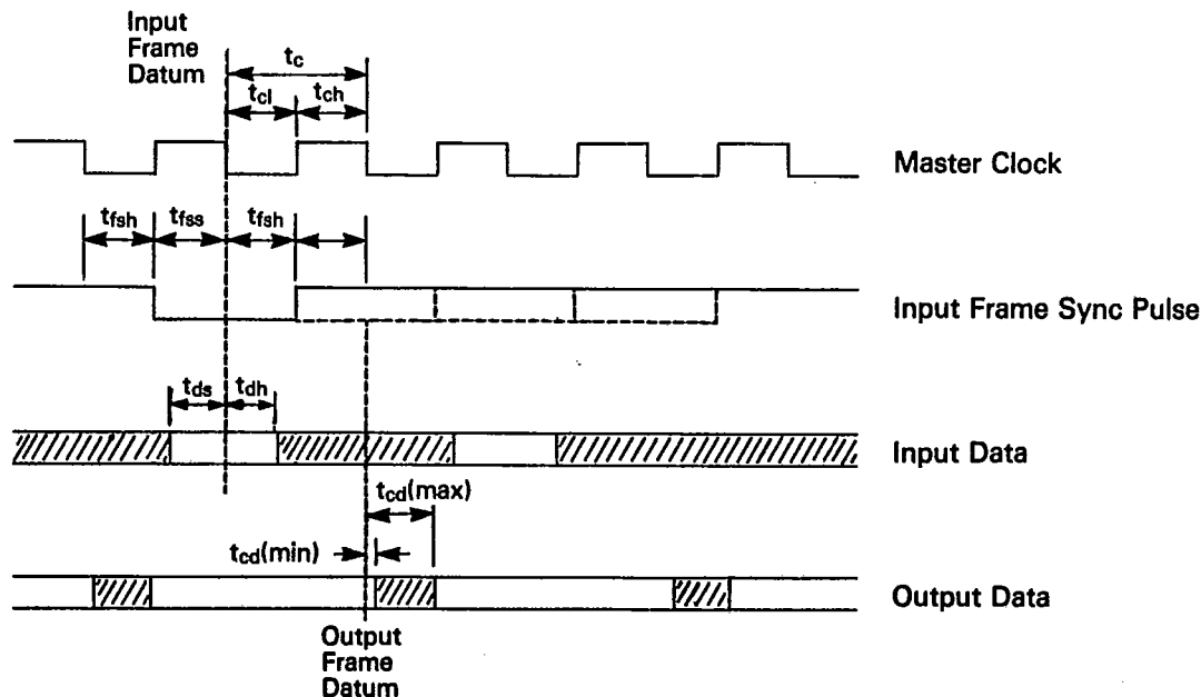
Figure 3(b) TIMING INFORMATION
