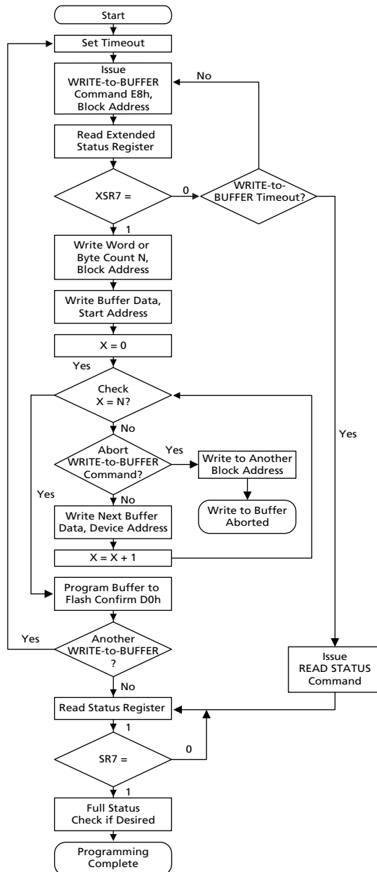
Figure 4 WRITE-to-BUFFER Flowchart
