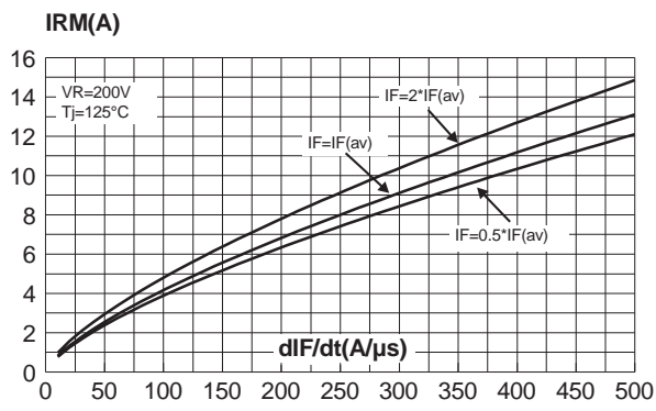
Fig. 4: Peak reverse recovery current versus di_F/dt (90% confidence, per diode).
