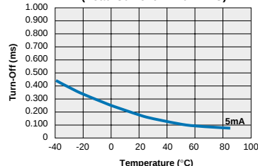
TS120 Typical Turn-Off vs. Temperature (Load Current = 120mA)
