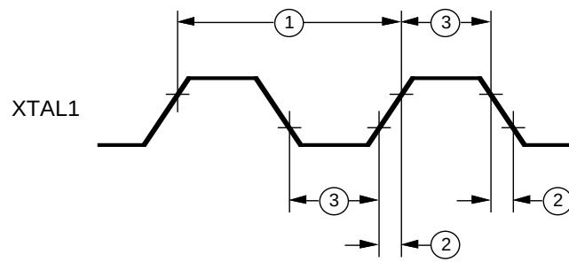
External Clock
