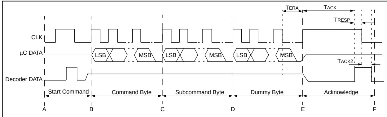
FIGURE 4-9: ERASE ALL
