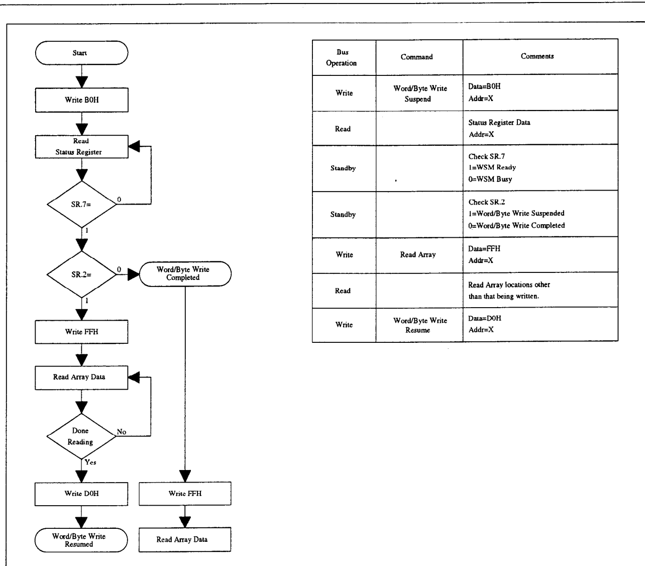
Figure 8. Word/Byte Write Suspend/Resume Flowchart
