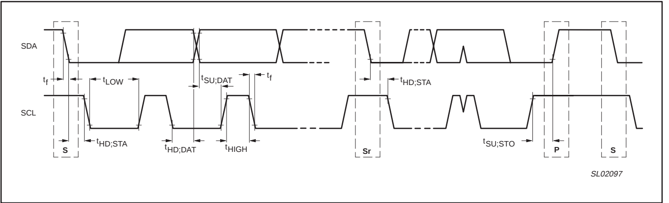
Figure 4. Timing diagram.
