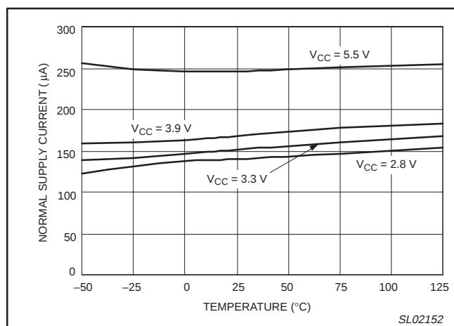
Figure 6. Typical normal I^2\text{C} inactive supply current versus temperature and V_{CC}
