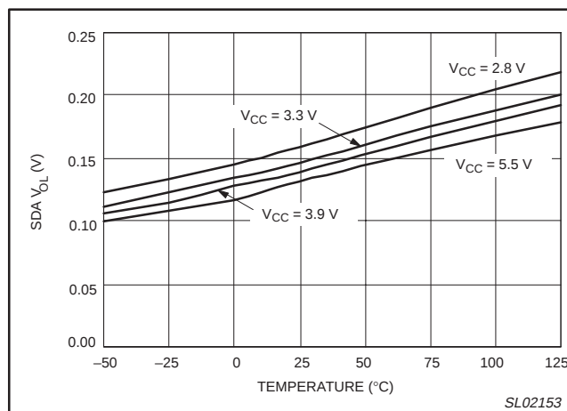
Figure 8. Typical SDA V_{OL} versus temperature and V_{CC} ( I_{OL} = 3 \text{ mA} )
