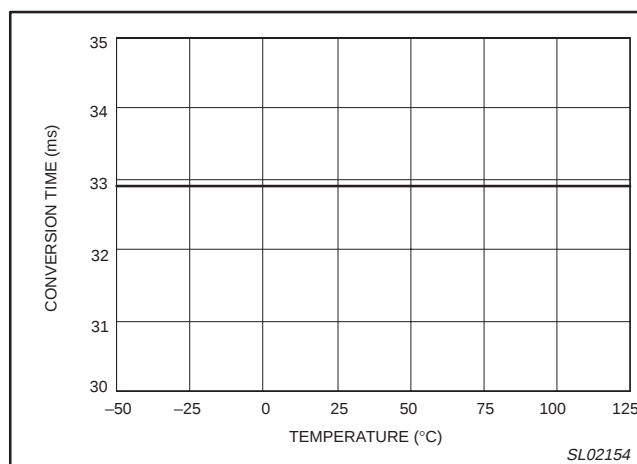
Figure 9. Typical conversion time versus temperature ( V_{CC} = 2.8 \text{ V to } 5.5 \text{ V} )
