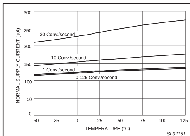
Figure 7. Typical normal I^2\text{C} inactive supply current versus temperature and conversion rate ( V_{CC} = 3.3 \text{ V} )
