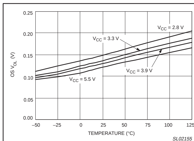
Figure 10. Typical OS V_{OL} versus temperature and V_{CC} ( I_{OL} = 3 \text{ mA} )
