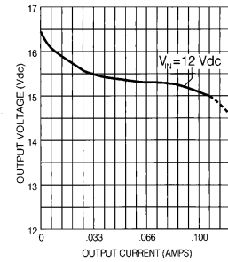
Output Current vs Output Voltage DCH1215D FIGURE 5
