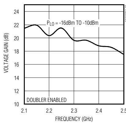
MIXER VOLTAGE GAIN vs. FREQUENCY vs. LO POWER
