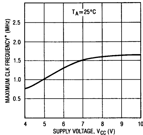
Maximum Clock Rate vs Supply Voltage
