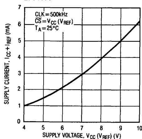
Supply Current vs Supply Voltage LTC1091
