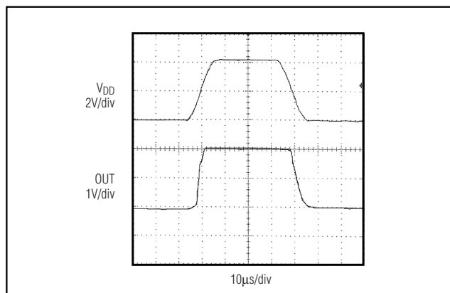
Figure 5. Power-Up/Power-Down Waveform
