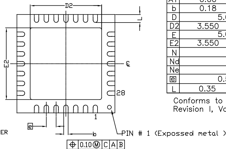
BOTTOM VIEW
