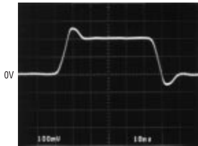
5V Small-Signal Response
