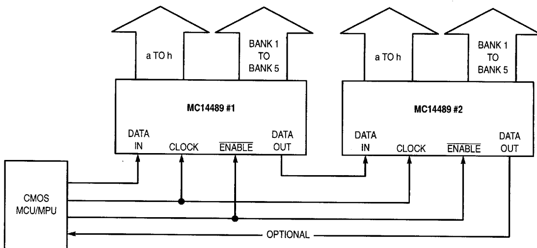
Figure 11. Cascading Two Devices
