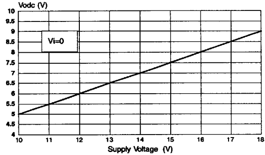
Output DC Voltage vs. Supply Voltage
