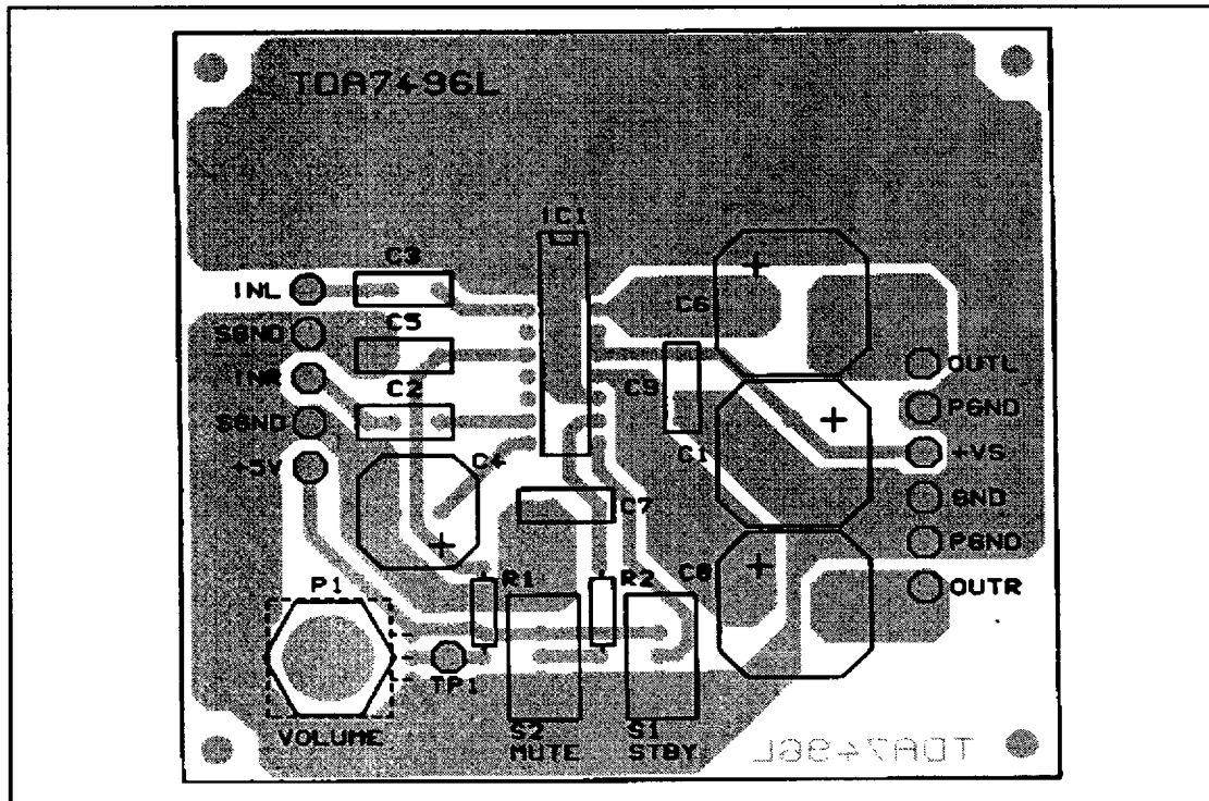
Figure 1B. PCB and Component Layout of the Fig. 1A (1.25:1 scale)
