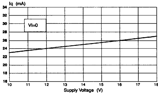
Quiescent current vs. Supply Voltage
