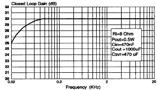
Closed Loop gain vs. Frequency
