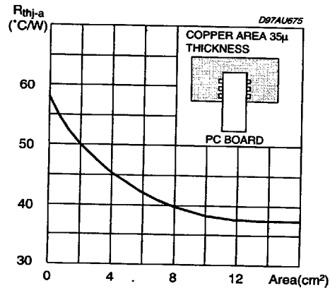
Rth with "on board" Square Heatsink vs. copper area.
