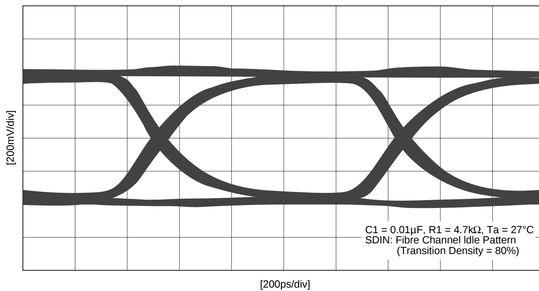
Eye pattern (Retimed data 1.0625Gbps)
