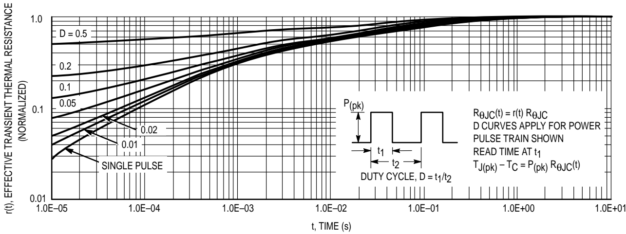
Figure 14. Thermal Response
