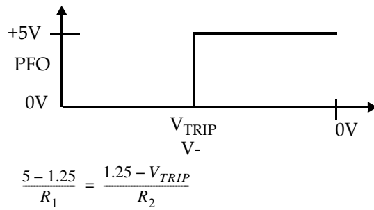
Figure 8: Using PFI To Monitor Negative Supply Voltage
