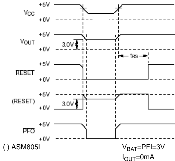
Figure 1: RESET/ \overline{RESET} Timing
